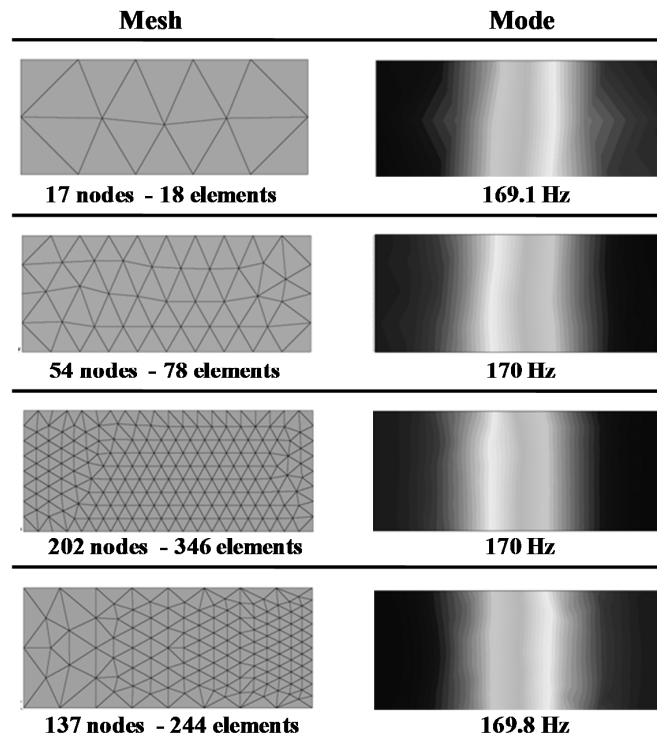
Figure 3 Rectangular cavity results. Meshes at left. Pressure distribution for the 1 th mode at right.
