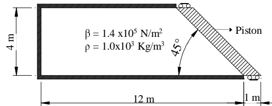
Figure 5 Skewed cavity coupled with movable piston.
