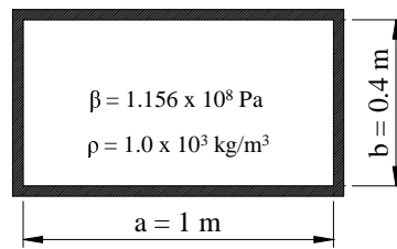
Figure 2 Rectangular cavity. Dimensions and fluid properties.
