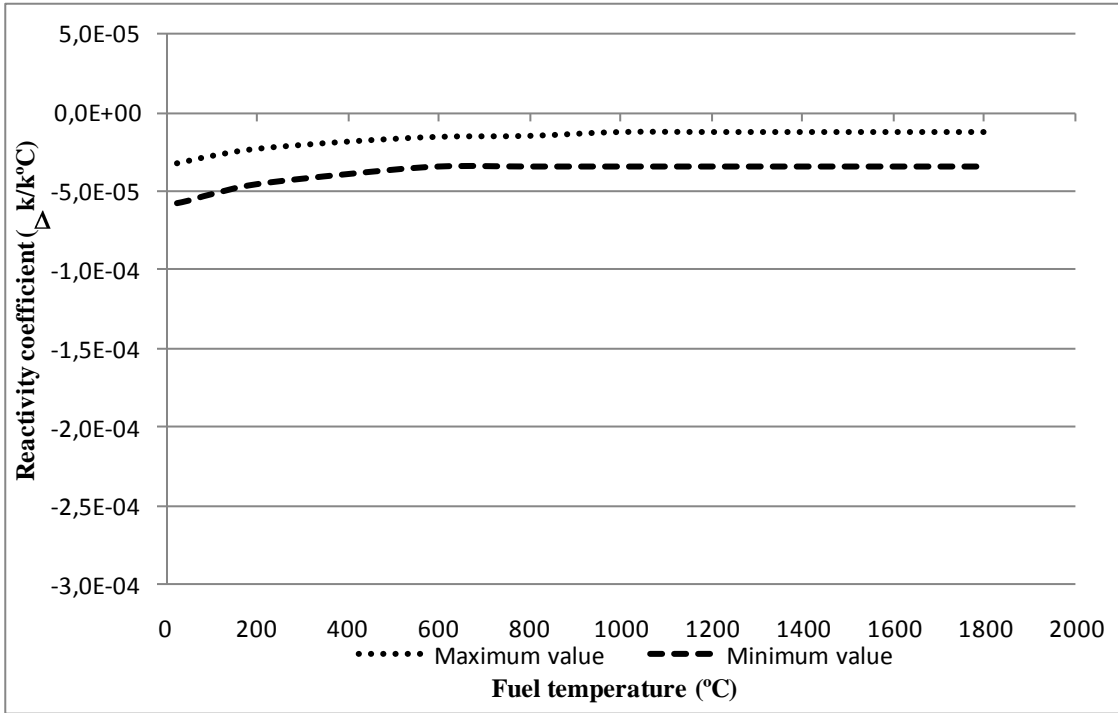
Fig. 3. Doppler coefficient.
