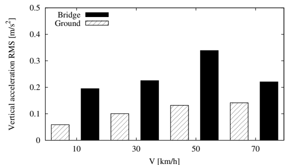
Figure 16. RMS of vertical acceleration without road roughness on the bridge and on the road.
