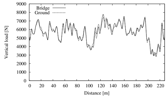
Figure 15. Vertical reaction in the windward rear wheel on the bridge and on the road ( U=20 m/s - V=70 km/h).
