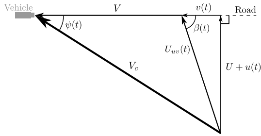
Figure 4. Relative wind velocity in the vehicle.
