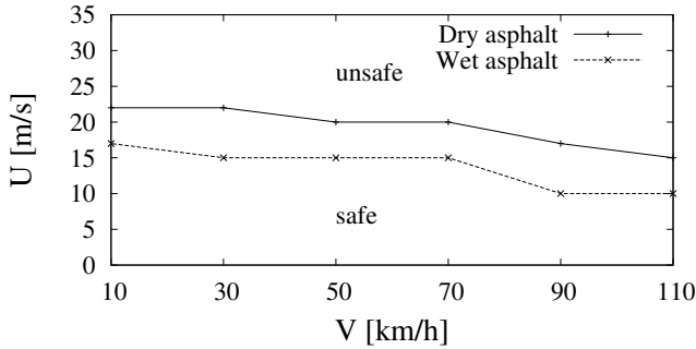
Figure 6. CWC in a rigid road without roughness.
