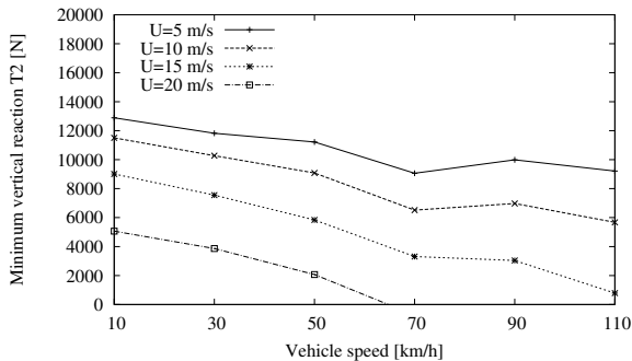
Figure 13. Minimum vertical load under rear windward tyre in a rigid road with roughness (IRI=2.0 dm/hm).
