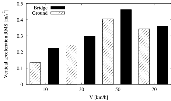
Figure 17. RMS of vertical acceleration with road roughness (IRI=2.0 dm/hm) on the bridge and on the road.
