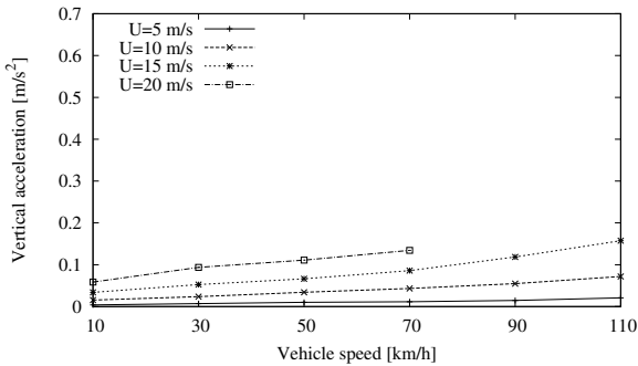
Figure 7. Vehicle vertical acceleration RMS in a rigid road without roughness.
