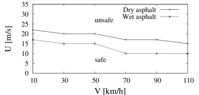
Figure 10. CWC in a rigid road with roughness (IRI=2.0 dm/hm).
