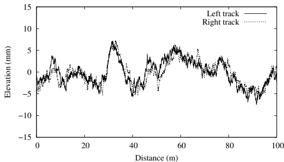
Figure 3. Parallel profiles at a distance of 2.20 m.
