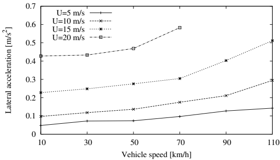
Figure 12. Vehicle lateral acceleration RMS in a rigid road with roughness (IRI=2.0 dm/hm).
