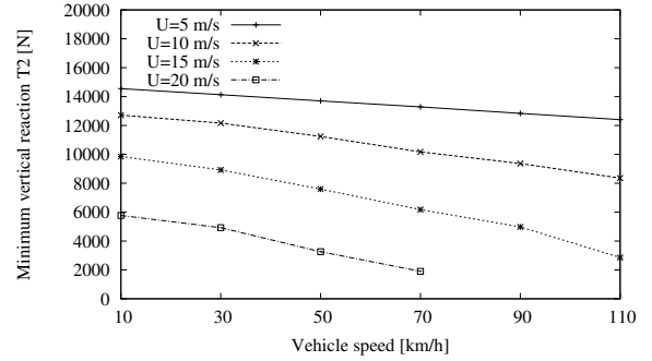
Figure 9. Minimum vertical load under rear windward tyre in a rigid road without roughness.
