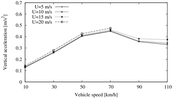
Figure 11. Vehicle vertical acceleration RMS in a rigid road with roughness (IRI=2.0 dm/hm).
