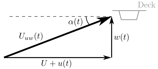
Figure 5. Wind velocity in the deck.
