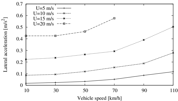
Figure 8. Vehicle lateral acceleration RMS in a rigid road without roughness.
