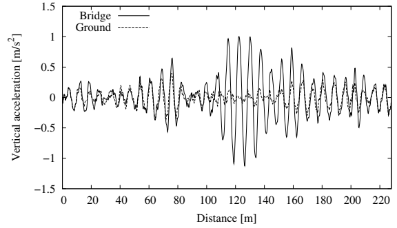
Figure 14. Vertical acceleration in the vehicle on the bridge and on the road ( U=20 m/s - V=50 km/h).
