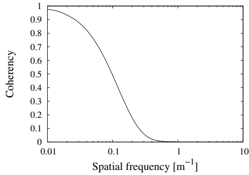
Figure 2. Coherency for vehicle width (2.20 m).
