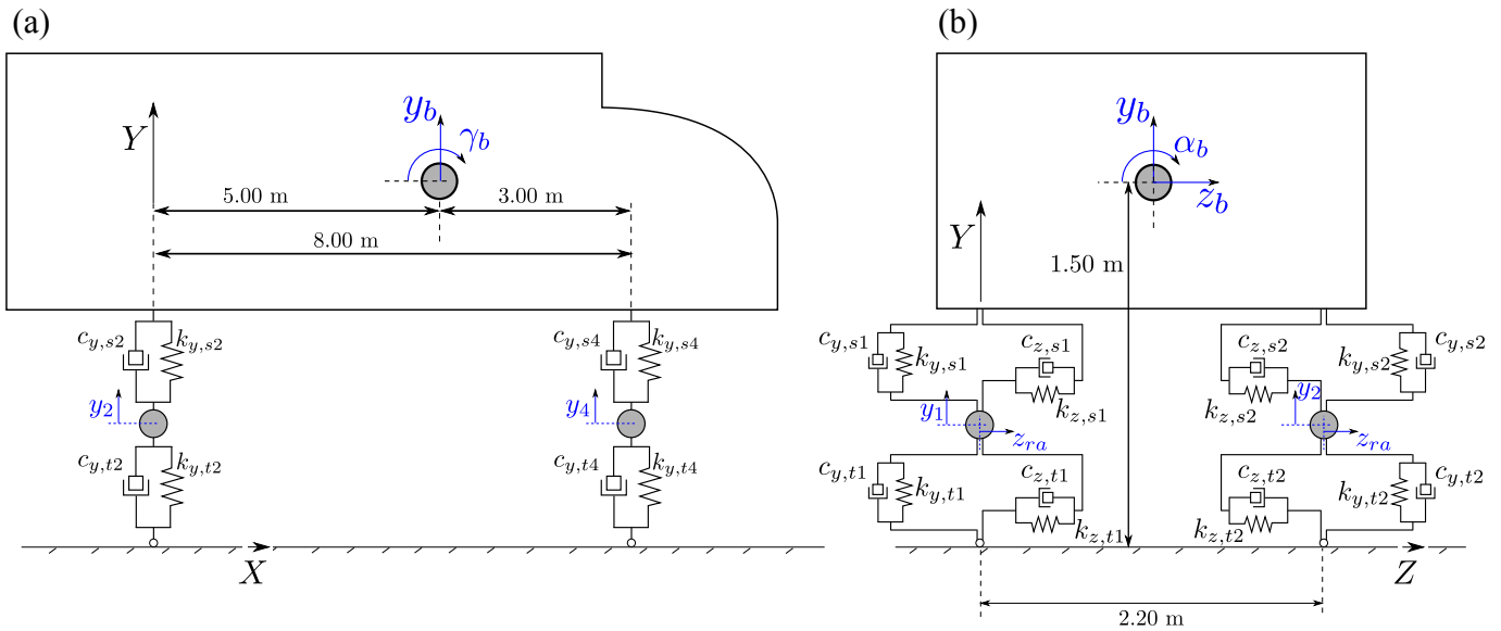
Figure 1. Vehicle model: (a) Side view; (b) Rear view.
