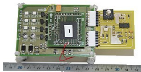
Fig. 1. Node implementation
