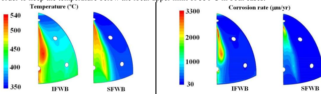
Fig. 4. Temperature and corrosion rates maps of the IFWB and the SFWB
