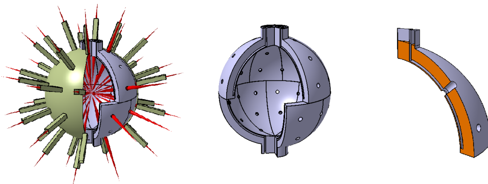
Fig. 1. Blanket and vacuum chamber of HiPER reactor
