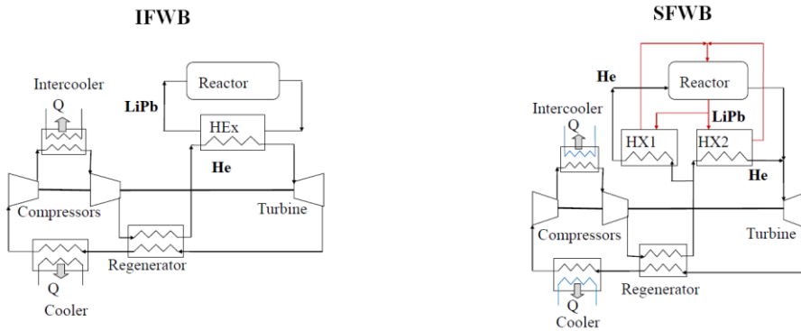
Fig. 3. Helium Brayton power cycle for the SCLL blanket of HiPER reactor
