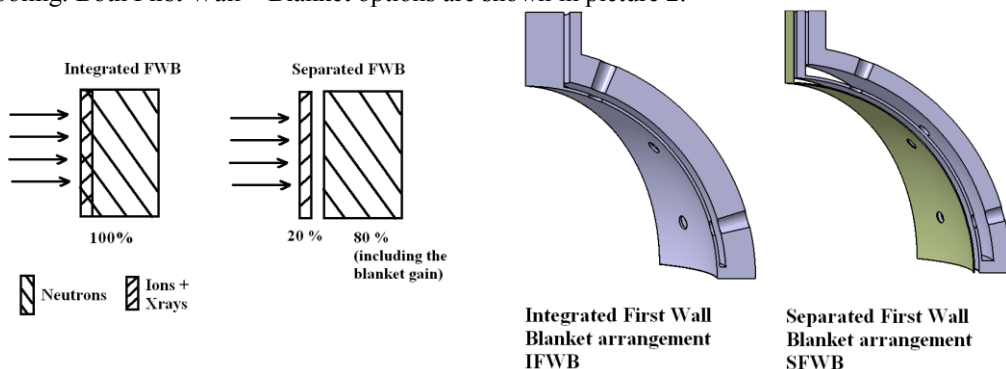
Fig. 2. Neutron, ion and X-Ray energy deposition in IFWB and SFWB
