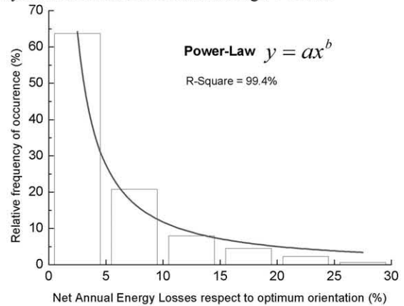
Figure 5: Proportion of PV systems (in %) oriented so that they lose less than a given percentage of net annual energy respect to the optimum orientation. Almost 65% of the PV systems lose less than 5% of annual energy due to their orientation, and less than 10% lose more than 15%.
