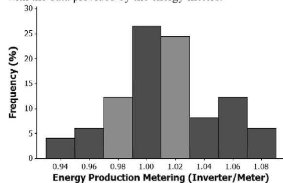
Figure 1: Histogram of the relation between the energy metering by inverter and meter
