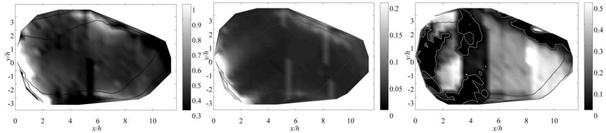
Figure 7: Surface distribution of mean pressure coefficient, C_p , (left), standard deviation pressure coefficient, C_{op} (middle), and skewness of the pressure, S_p , (right) along line A (239°), for a Reynolds number Re_h = 5.1 \times 10^4 . The dark lines indicate isocline curves, and the white lines indicates the loci where S_p = 0 on the surface
