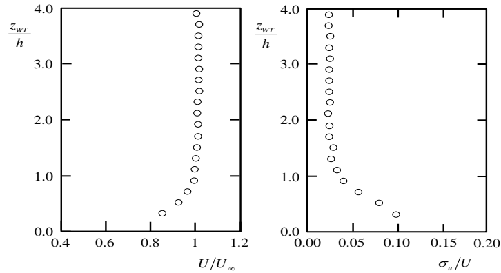
Figure 4: Vertical profiles of mean wind speed and turbulence intensity at x_{WT}/h=0 , at y_{WT}/h=0 . Conditions measured without the mock-up.
