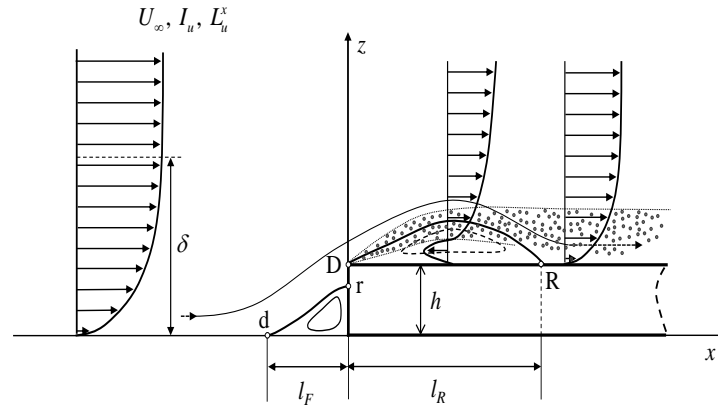
Figure 1: Schemantic of the ensemble mean flow velocity field around a 2D-truly isolated FFS (adapted from Sherry et al., 2010 and Bradshaw & Wong, 1972). d : mean position of the detachment point in front of the FFS, r : mean position of the reattachment point on the vertical wall, D : position of the detachment point on top of the FFS (edge), R : mean position of the reattachment on top of the FFS. l_F is the mean length of the front separation bubble and l_R is the mean length of the separation bubble on top of the FFS. The shear layer originated at D is schematised with grey dots.
