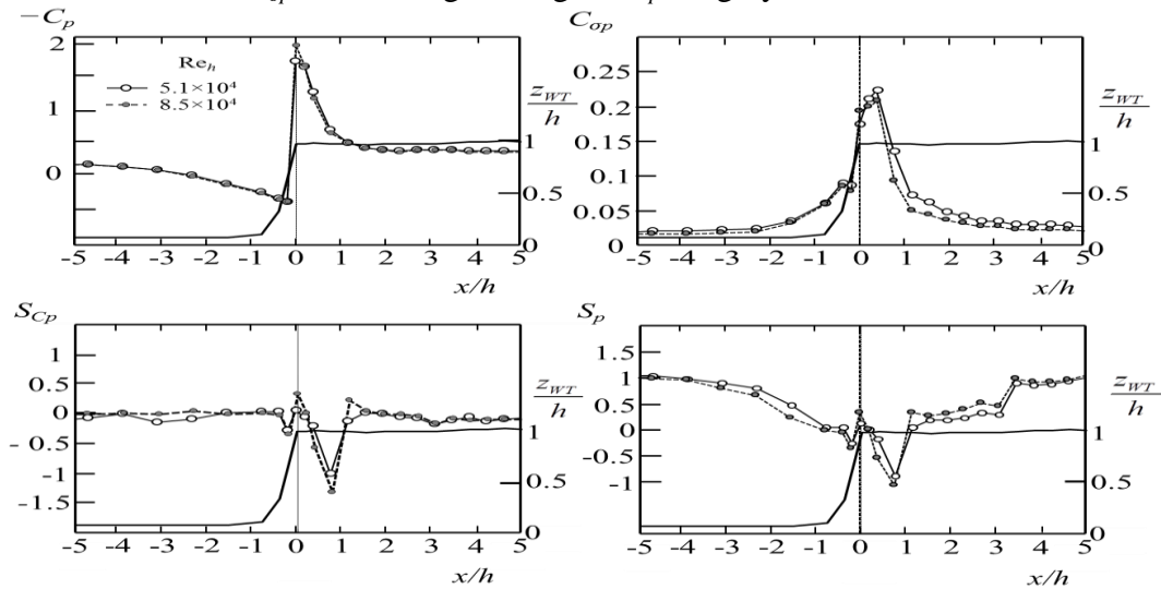
Figure 5: Distribution of mean pressure coefficient, C_p , expression (0.1), standard deviation pressure coefficient, C_{op} , expression (0.2), Skewness of pressure coefficient, S_{Cp} , and skewness of the pressure, S_p , expression (0.3) along line B ( 270^\circ ), for two Reynolds numbers, Re_h , indicated in the figure. The profile of the island for the mentioned direction is shown in the figure in continuous line.
