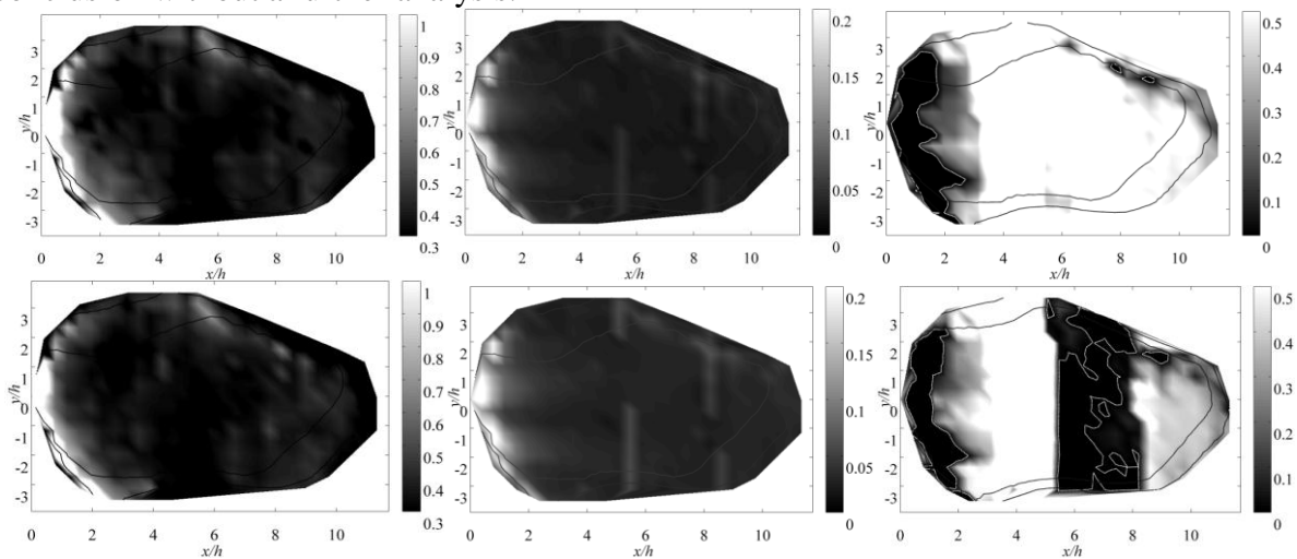
Figure 6: Surface distribution of mean pressure coefficient, C_p , (first column), standard deviation pressure coefficient, C_{op} (second column), and skewness of the pressure, S_p , (third column) along line B ( 270^\circ ), for two Reynolds numbers (top row, Re_h = 5.1 \times 10^4 , bottom row, 8.5 \times 10^4 ). The dark lines indicate isolevel curves, and the white lines indicates the loci where S_p = 0 on the surface.
