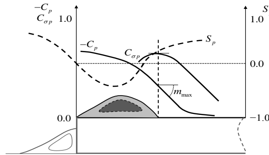
Figure 2: Schematic on the diagnostic process on the bubble length l_R/h based on the behaviour of the mean pressure coefficient, C_p , the std. pressure coefficient, C_{op} , and the skewness of the pressure, S_p .
