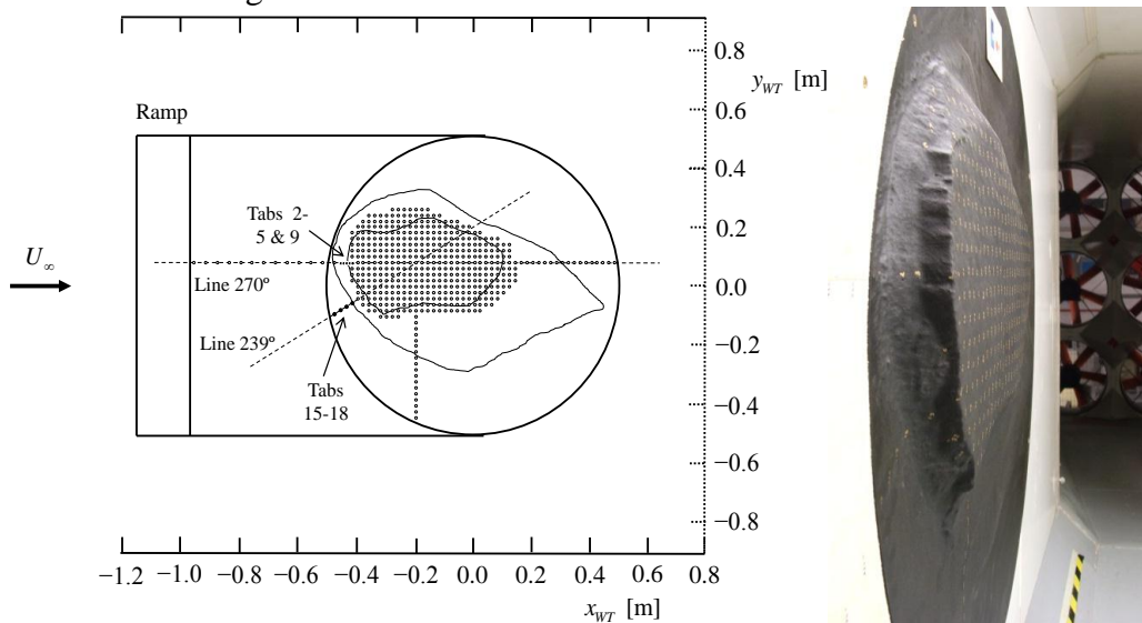
Figure 3: Pressure tabs distribution on the island model and schematic of the mounting in the A9 wind tunnel.
