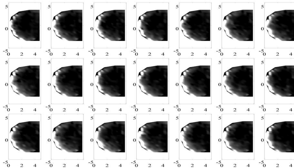
Figure 8: Surface distribution of the instantaneous pressure coefficient, -\tilde{c}_p , for the case 270° and a Reynolds number Re_h=8.5 \times 10^4 . The color bar is the same as for the C_p figures in figure 15 and 16.
