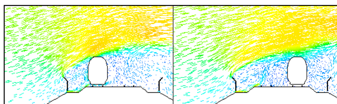
Figure 6: Displays of velocity vectors for one of the simulations. The trains are SIEMENS type, and the barriers were the optimum obtained for embankment.
