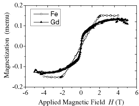
FIG. 6. Hysteresis loop with the field applied perpendicular to the sample plane for a thin film of Ta(3 nm)/Fe(6 nm)/Ta(3 nm) (circles) and a thin film of Ta(3 nm)/Gd(4 nm)/Ta(3 nm) (triangles), measured at 10 K.
