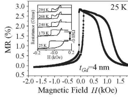
FIG. 3. MR loop for the sample with 4 nm of Gd at 25 K. The shape of this loop is very similar to the one shown in Fig. 2(a) for no Gd, which shows that the two Fe layers are exchange coupled through the Gd. The inset shows a sequence for several temperatures for a low-field zoom of the loop. The vertical scale of the inset is shown on its right.
