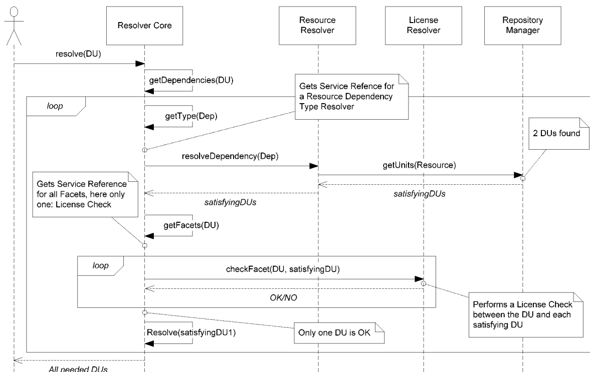
Figure 4: Dependency Resolution.
