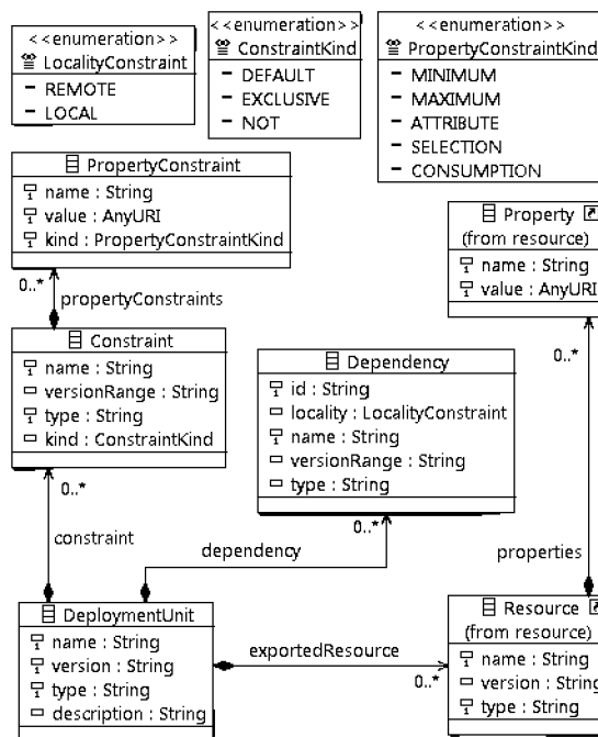
Figure 1: Software component metamodel.
