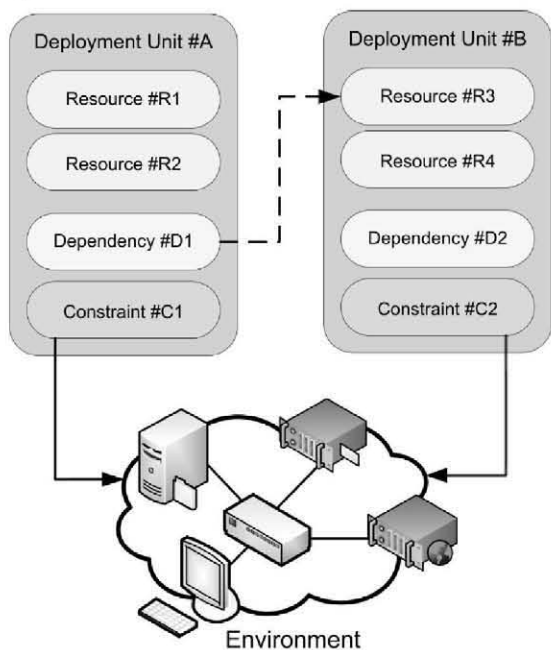
Figure 2: Dependencies and Constraints.
