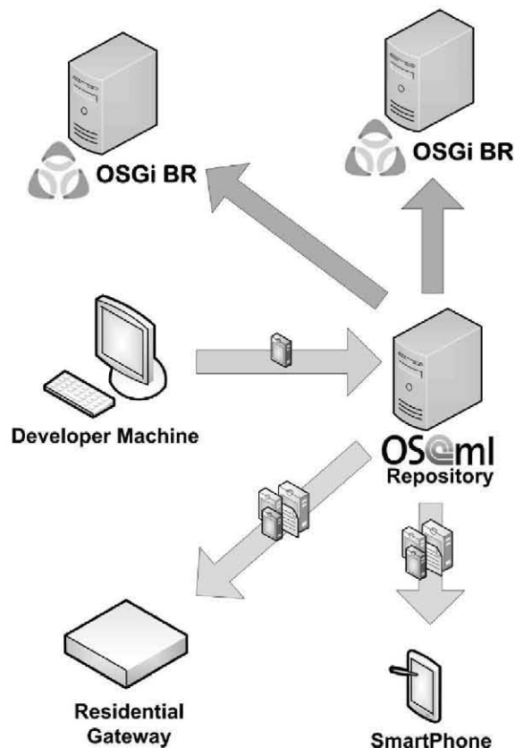
Figure 5: Repository Federation.
