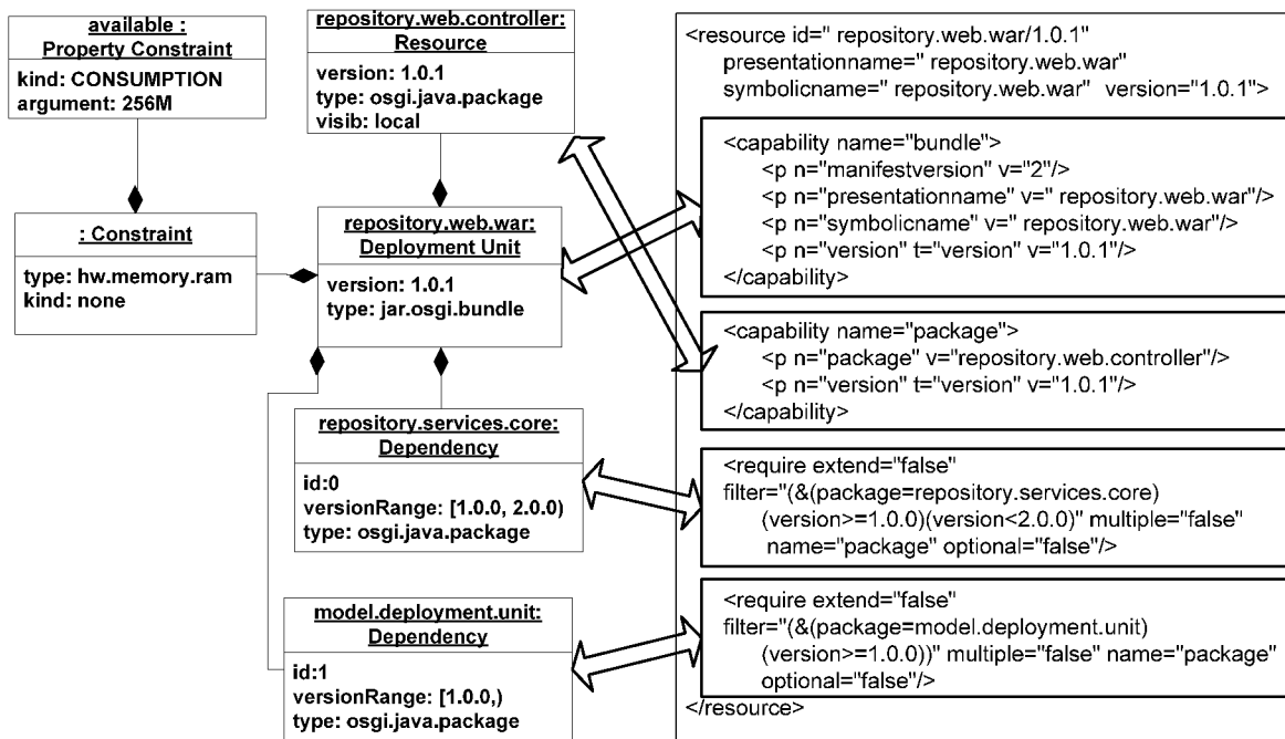
Figure 6: Model mapping between OBR and the presented model.
