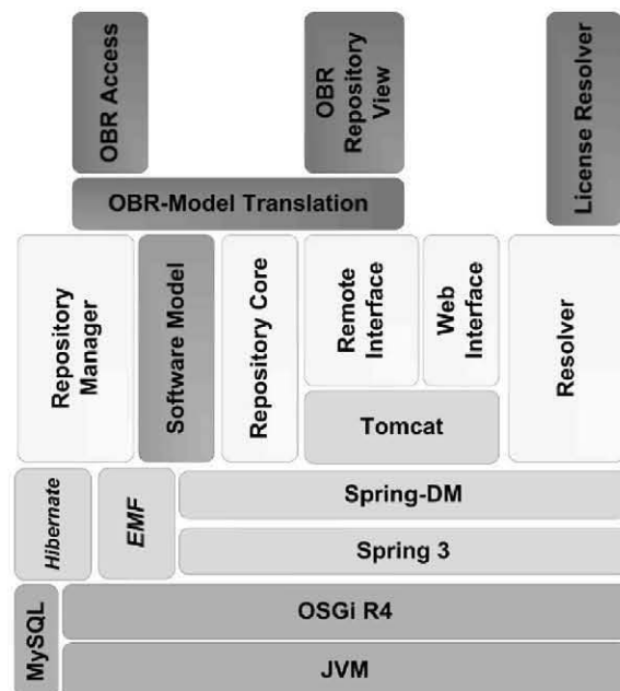
Figure 3: Repository Architecture.
