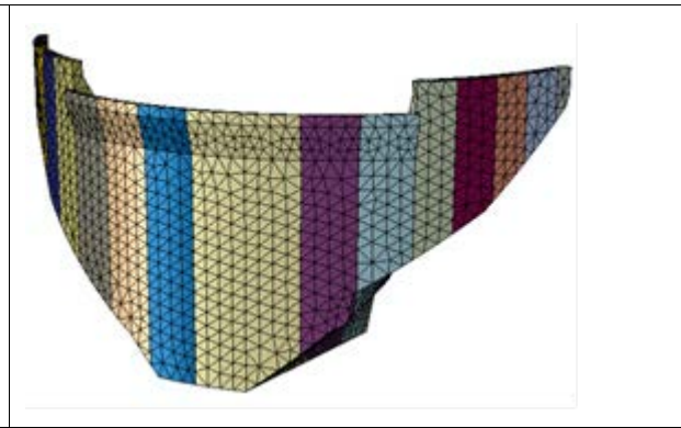
Figure 7: Mesh of the arch gravity dam
