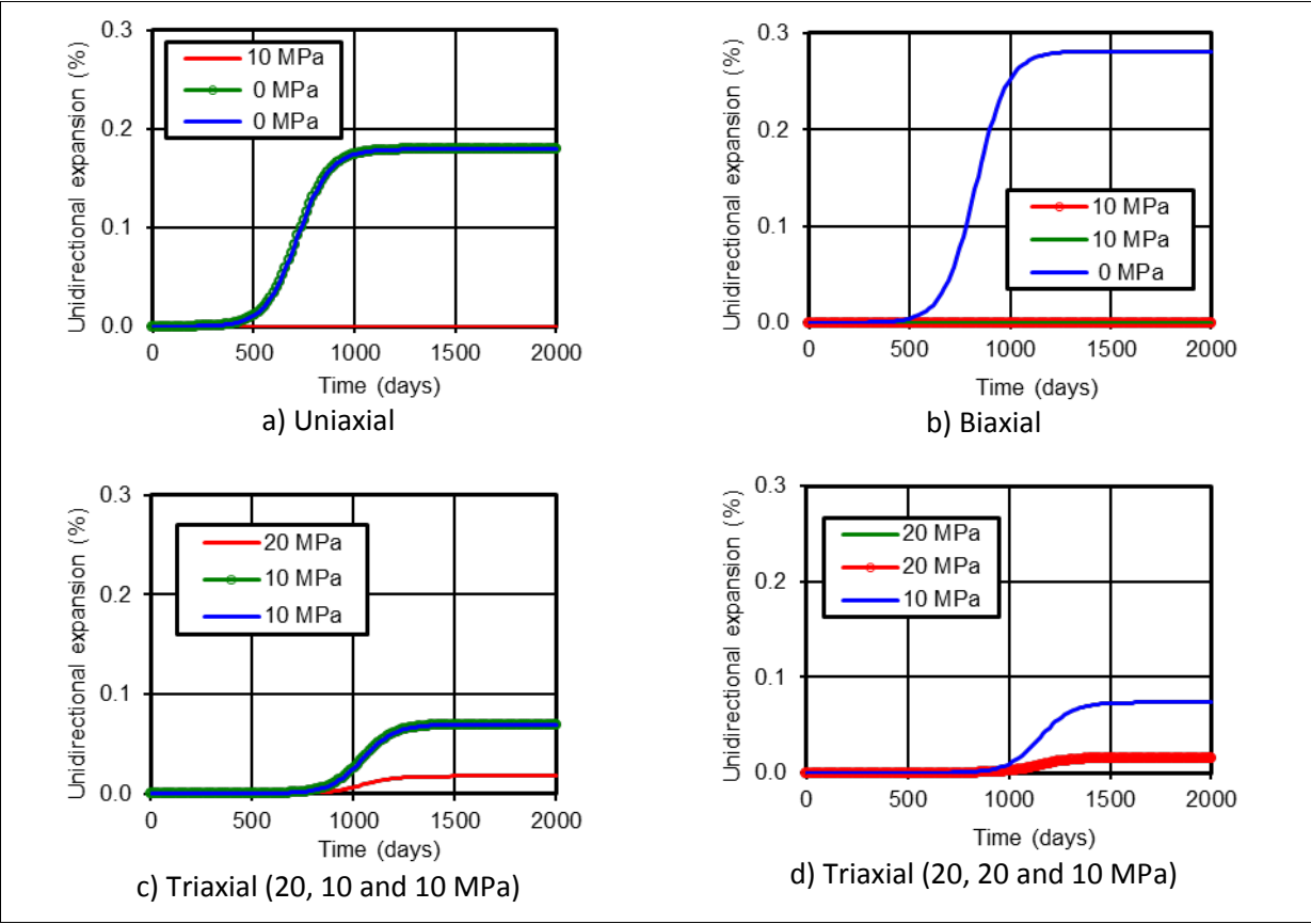
Figure 4: Unidirectional expansion
