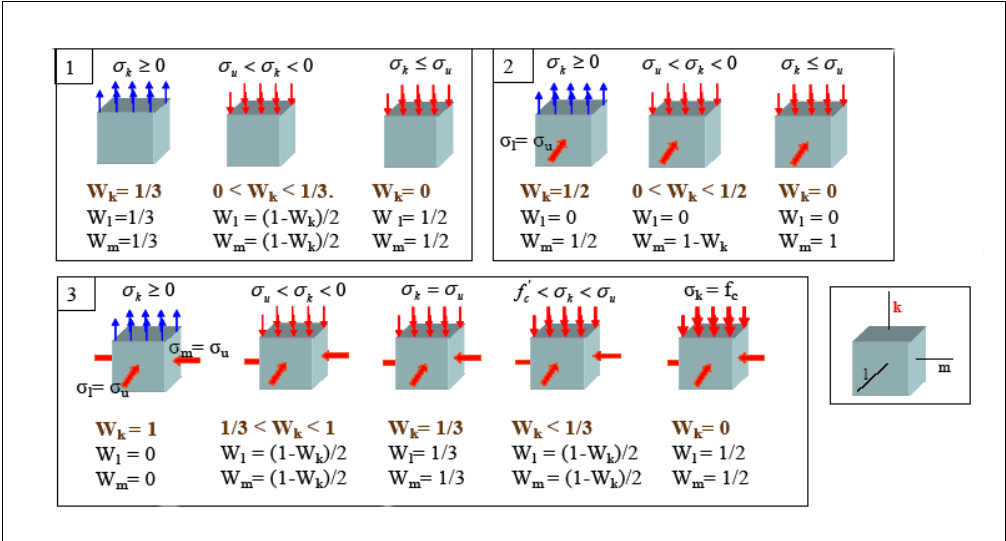
Figure 2: Distribution of expansion after Saouma and Perotti
