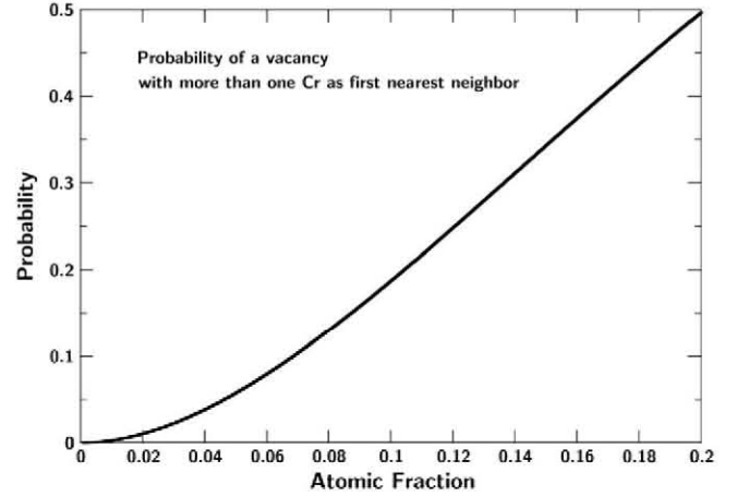
Fig. 7. Probability of having more than one Cr atom at first nearest neighbor distance of a vacancy as a function of Cr concentration in FeCr random solution.
