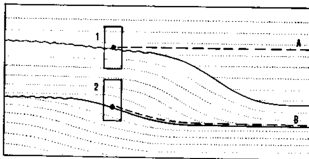
Fig. 3. Sketch representing several transgression—regression cycles with two ruptures dividing the record into three tecto-sedimentary units
