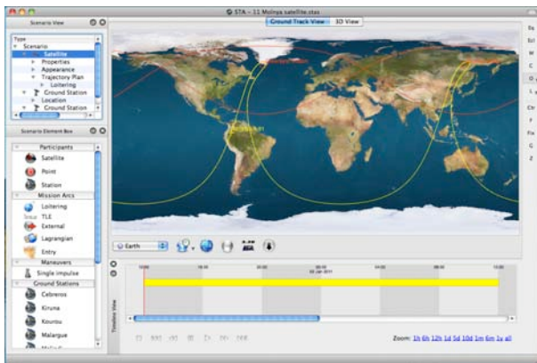
Figure 11. Scenario of a Molnya orbit
