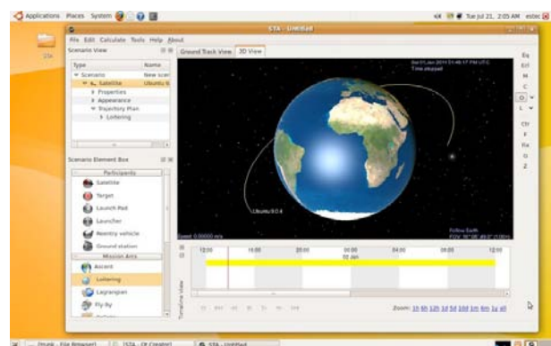
Figure 1. STA screenshot
