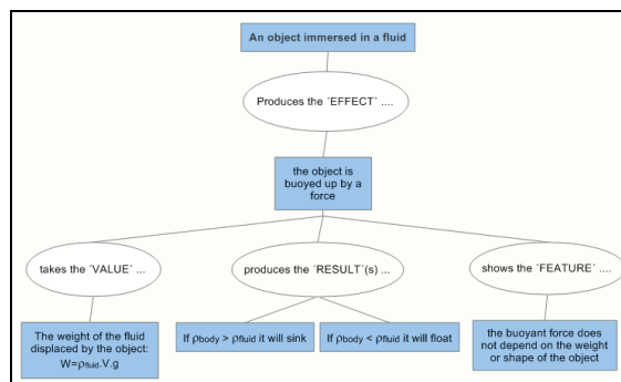
Figure 1: Archimedes Principle.
