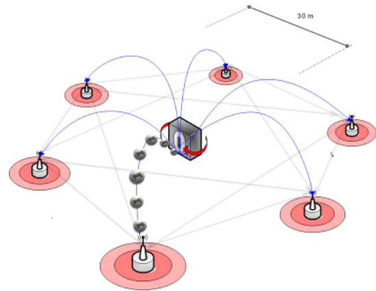
Figure 5. WSN star topology with rover as sink node.
