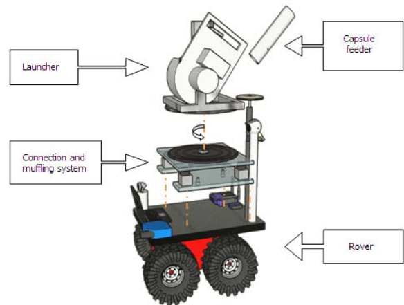
Figure 9. Mobile deployment engine design.
