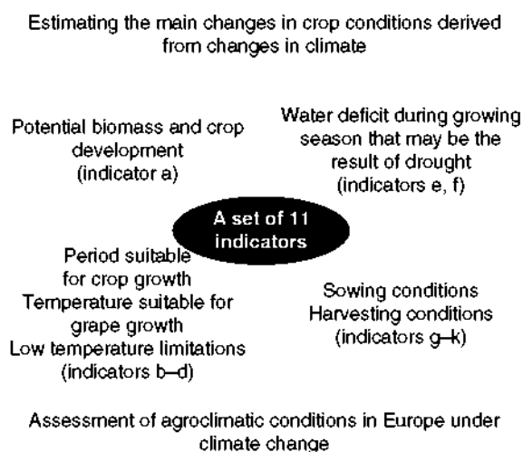
Fig. 2 Overview of the methodological approach to using indicators for the evaluation of changes in agroclimatic conditions in Europe under climate change.
