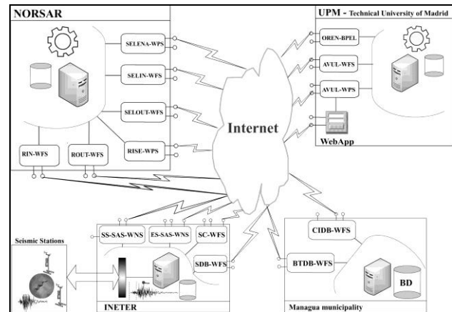
Figure 2. System architecture proposed for the web services
