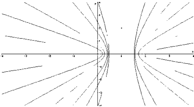
Fig. 1: Regions for capturing the maximum number of voters when the parties agree on one of the policies they offer
