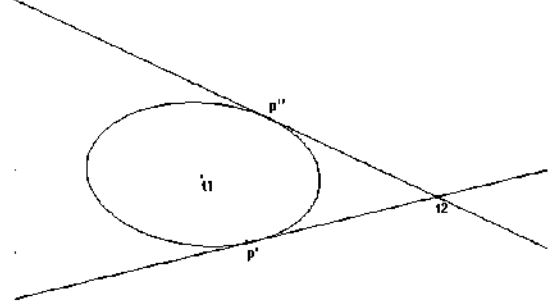
Fig. 2: The arc delimits an area with maximum votes for t_1 .
