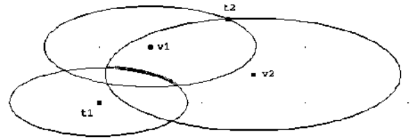
Fig. 3 The marked arc represents the area on the border of N_1 with maximum votes for t_1 given points v_1, v_2 .
