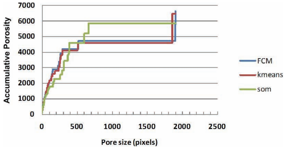
Fig. 6. Pore space distribution for the A2 horizon.
