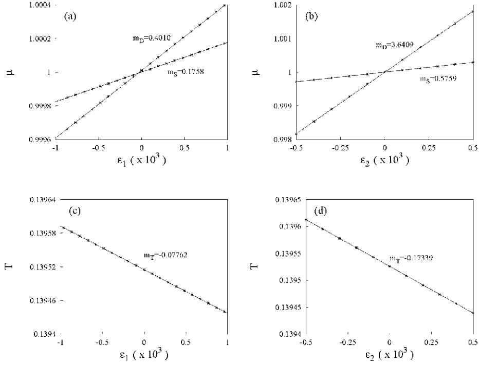
FIGURE 9. Linear dependence of the leading Floquet multipliers near the multi-critical point versus the unfolding parameters: a) \varepsilon_1 , and (b) \varepsilon_2 . Linear dependence of the period T , (c) on \varepsilon_1 , and (d) on \varepsilon_2 .
