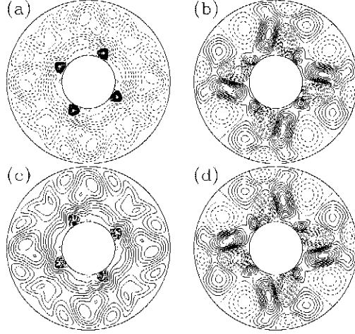
FIGURE 8. From left to right, (a), (b) instantaneous streamlines, and temperature perturbation, respectively, for U_5(0) , and (c), (d) for U_5(T/2) . Ro_c = 10385 , \eta_c = 0.3255 .
