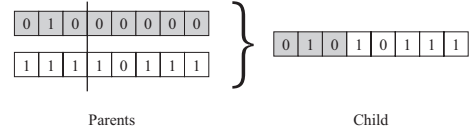
Figure 8. Single point crossover.
