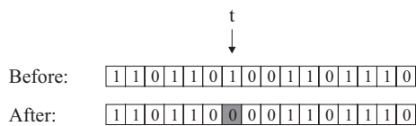
Figure 10. Mutation.
