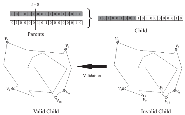
Figure 9. Single point crossover and validation.
