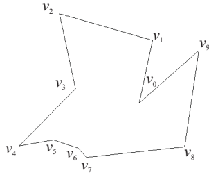
Figure 7. Polygon with n = 10 .
