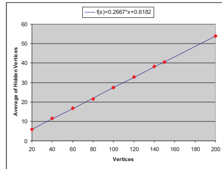
Figure 12. Least Squares Method.
