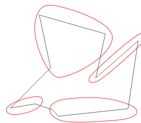
Figure 3. A clique partition (with 4 cliques) of VG(P) .
