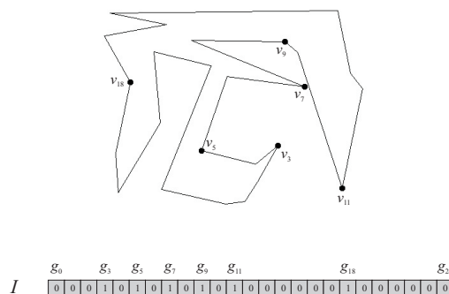
Figure 6. An individual, I , (for a polygon with n = 25 ) and its representation. Black dots represent hidden vertices.
