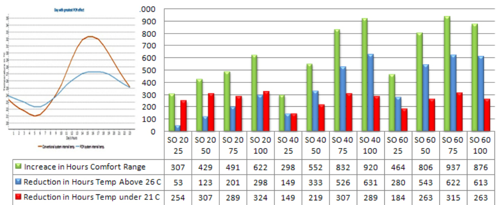
Figure 9. Soria with PCM Annual Results and SO6075 chart of interior temperatures on July 9.
