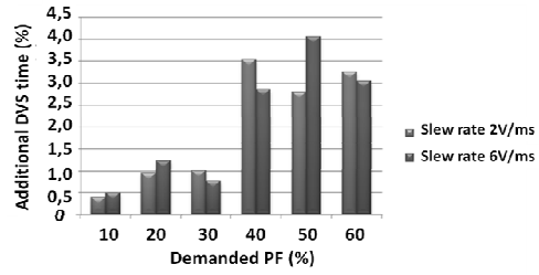
Fig. 11 Additional DVS time for different slew rates of the power supply
