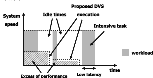
Fig.1 DVS using CPU's idle times
