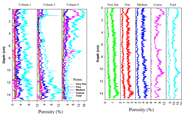
Fig.6. Range of soil porosity for each pore size in 12 columns
