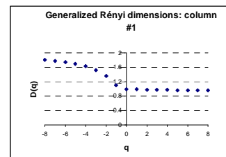
Fig.7. Generalized Rényi dimensions of the variation of 2D sectional porosity with depth
