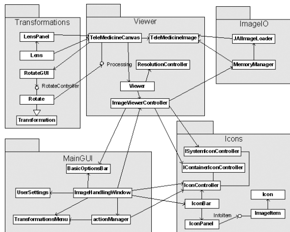
Figure 3. Recovered Architecture Diagram
