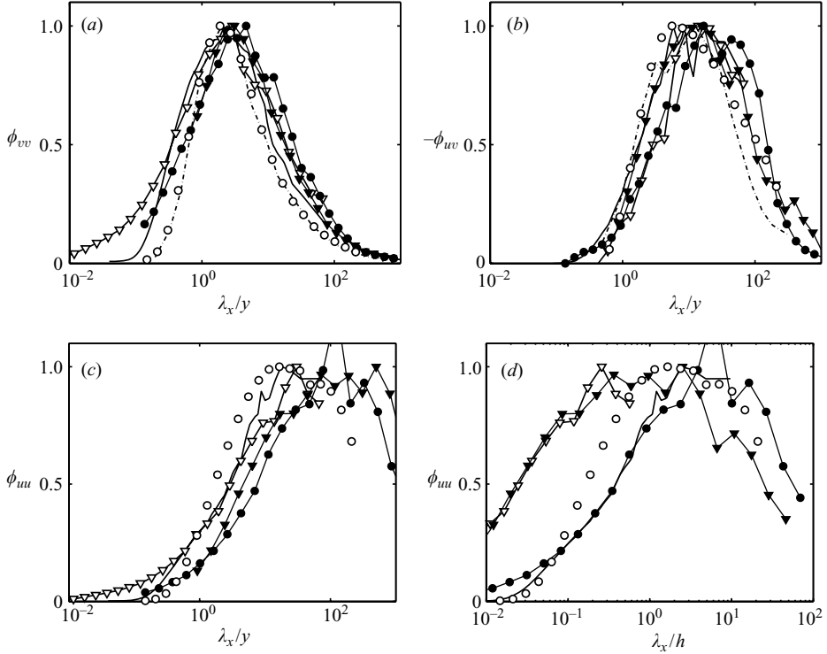
FIGURE 6. One-dimensional premultiplied spectra of (a) wall-normal velocity versus \lambda_x/y , (b) cospectrum -\phi_{uv} versus \lambda_x/y , (c) streamwise velocity versus \lambda_x/y , (d) streamwise velocity versus \lambda_x/h , in the logarithmic layers of experimental and atmospheric flows. The spectra are normalized to unit maxima, because of the uncertainty in the actual Reynolds stresses. \blacktriangledown , ABL, y = 1 m, u_\tau = 0.65 m s ^{-1} , h = 200 m (Hoxey & Richards 1992); \bullet , same case y = 10 m; \nabla , ABL, y = 1.7 m, u_\tau = 0.24 m s ^{-1} , h = 200 m (Antonia & Pearson 1999); —, boundary layer, y/h = 0.14 , Re_\tau = 7000 (Carlier 2001); - - -, pipe, y/h = 0.12 , Re_\tau = 2100 (Lawn 1971); \circ , channel L2000, y/h = 0.1 . Both ABLs are fully rough.
