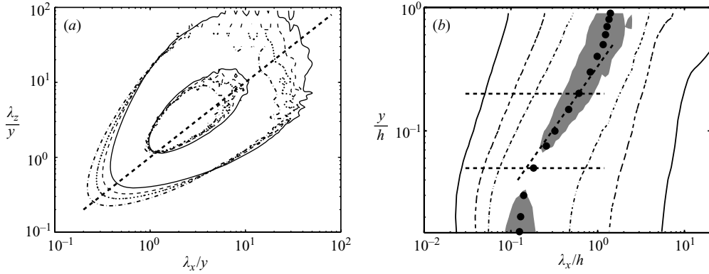
FIGURE 9. Spectral density functions for the pressure fluctuations in case L2000. (a) As a function of \lambda_x/y and \lambda_z/y . —, y/h = 0.1 ; ----, y/h = 0.15 ; ·····, y/h = 0.2 ; — · —, y/h = 0.3 . The two contours in each spectrum are \phi_{pp}/\langle uv \rangle^2 = 0.125 and 0.625 times the common maximum of the four cases. (b) As a function of \lambda_x/h and y/h . Contours are \phi_{pp}/p'^2 = 0.03, 0.09, 0.3 . The dashed horizontal limits, diagonal and closed circles, are as in figure 1.
