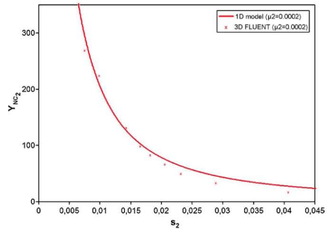
Fig. 25. Comparison of the non-dimensional centre line of the plume, for case 1, obtained with the one-dimensional model and the three-dimensional code.
