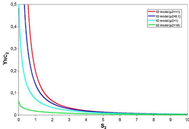
Fig. 23. Evolution of the mass concentration along the centre line for different values of \mu_2 obtained with the one-dimensional model for cases with upper cover. The 1D results are centre line values and the 3D results maximum values.
