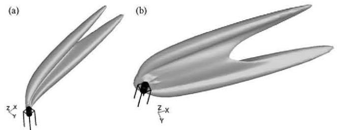
Fig. 11. Three-dimensional view of the cloud corresponding to a concentration equal to 5%. Mass flow rate is 70 kg/s and the wind velocity is v = 10 m/s: (a) without upper cover and (b) with upper cover.
