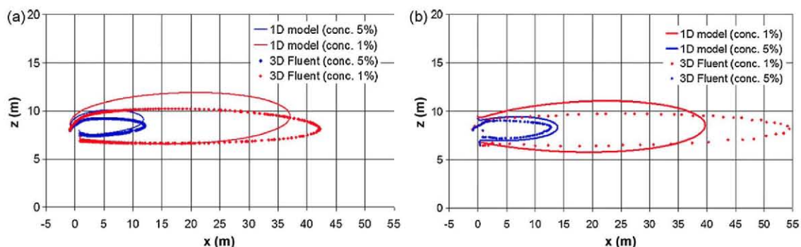
Fig. 12. Profiles of the plume, corresponding to a mass concentration equal to 1% and 5% (mass flow rate 5 kg/s, wind velocity 10 m/s). The numerical results obtained with the 1D and 3D model are compared. (a) Case without the upper cover and (b) case with the upper cover.
