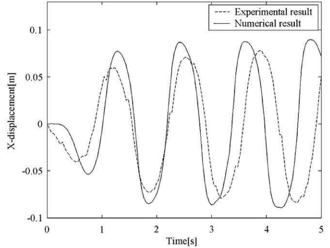
Fig. 9 Clamped elastic beam immersed in deep oil flow: comparison of the displacement in X direction
