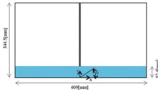
Fig. 10 Hanging elastic beam with shallow water: initial geometry and angle of the container versus time
