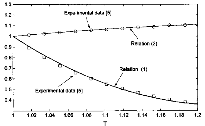
Fig. 2. Comparison between correlations generated for dynamic viscosity and thermal conductivity, and experimental data.
