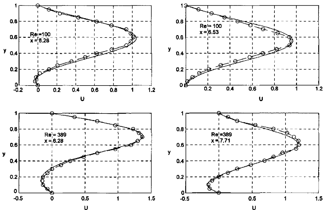
Fig. 4. Comparison between computed (–) and experimental (–o–) local velocity profiles at Reynolds 100 and 389 at different sections downstream of the step.
