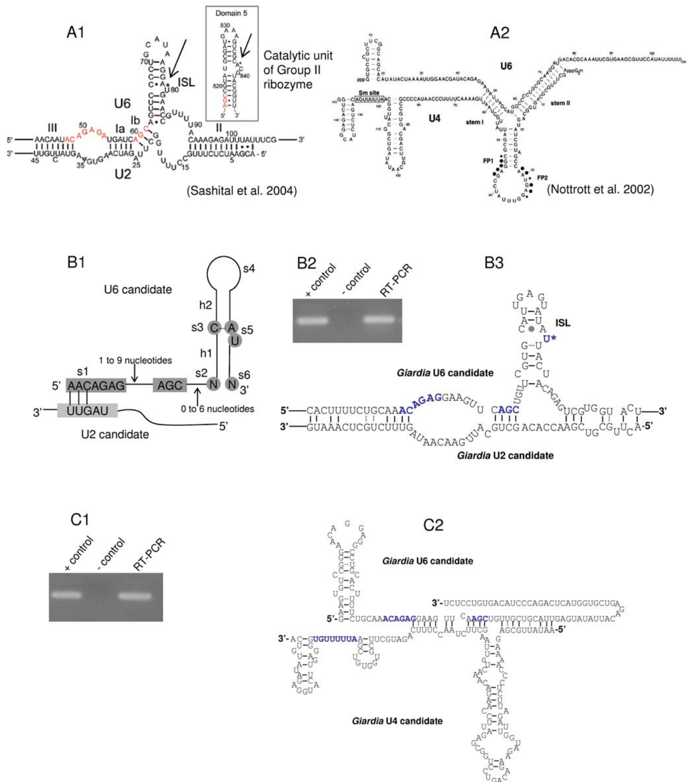
Figure 3. Identification of Giardia U6 and U4 snRNA candidates. A1. Structure of U2-U6-snRNA base pairing in S. cerevisiae . A2. Structure of U6-U4-snRNA base pairing in Human. B1. Visualization of the model for searching a U6-snRNA candidate. B2. RT-PCR test for expression of the U6 candidate. + control: PCR with genomic DNA. – control: PCR with total RNA without reverse transcription. B3. Interaction between Giardia U6 and U2 snRNA candidates. C1. RT-PCR test for expression of the U4 candidate. + control: PCR with genomic DNA. – control: PCR with total RNA without reverse transcription. C2. Interaction between Giardia U6 and U4 snRNA candidates. doi:10.1371/journal.pone.0003106.g003
