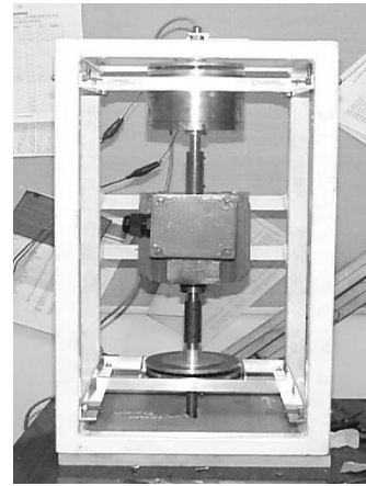
Fig. 10. Fabricated magnetic bearing system.
