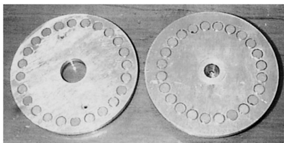
Fig. 3. Fabricated magnetic bearing.
