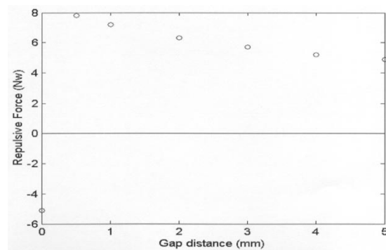
Fig. 11. Measured repulsive force characteristic.
