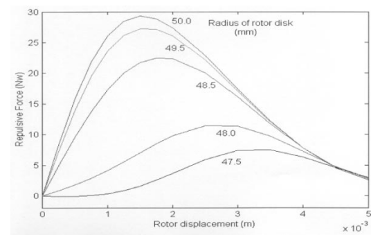
Fig. 6. Variation of repulsive force with radial displacement.
