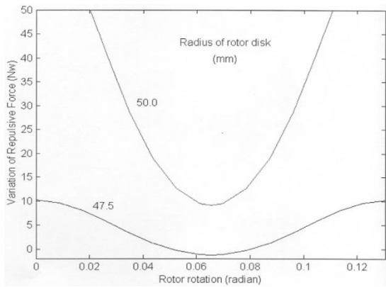
Fig. 7. Variation of repulsive force with rotor movement.
