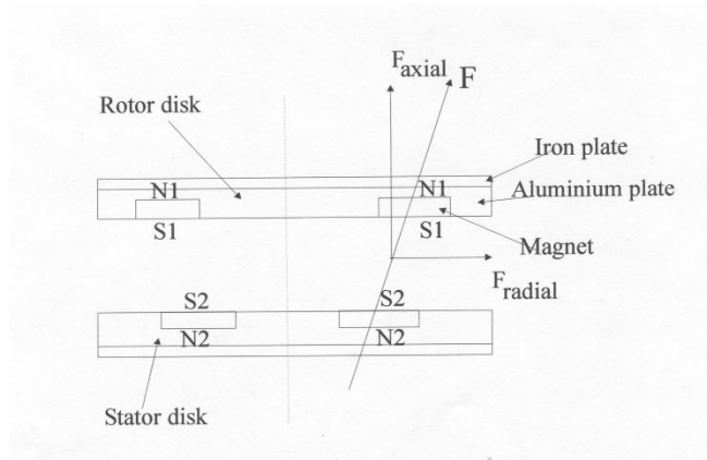
Fig. 2. Schematic representation of magnet arrangement and forces.
