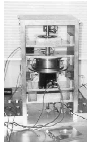
Fig. 1. Magnetic bearing for vertical shaft machine.
