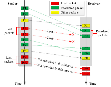
Fig. 1. The timeline of a measurement interval.
