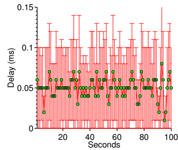
Fig. 10. One-way latency results between two servers reported by RDA based passive latency measurement software.
