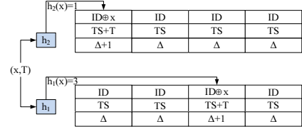
Fig. 5. RDA has multiple banks of buckets. A packet is inserted into a randomly selected bucket in each bank.
