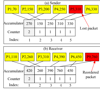
Fig. 2. An example of LDA that are damaged by problematic packets. The sender sends packets P1 to P9 to the receiver. A measurement interval begins before packet P1 and ends after packet P6. However, P5 is lost and thus not recorded at the receiver. Further, due to packet reordering, P9 arrives at the receiver earlier than the ending message, which is thus recorded at the receiver. In (a), the sender inserts the timestamps (shown in the upper-level box) of packets P1, P2, P3, P4, P5, P6 into its LDA. In (b), the receiver inserts the timestamps of packets P1, P2, P3, P4, P6 and P9 into its LDA.
