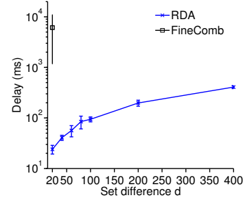
Fig. 6. The decoding time of RDA and FineComb.
