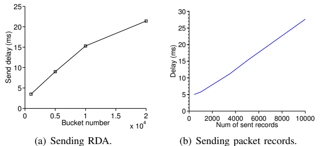
Fig. 14. The time of transmitting RDAs and that of sending the packet records that consist of the timestamps and identifiers of missing packets.
