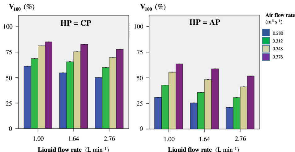
Fig. 12. V_{100} for different combinations of variables for the two positions of the liquid hose. The error bars indicate the standard errors.
