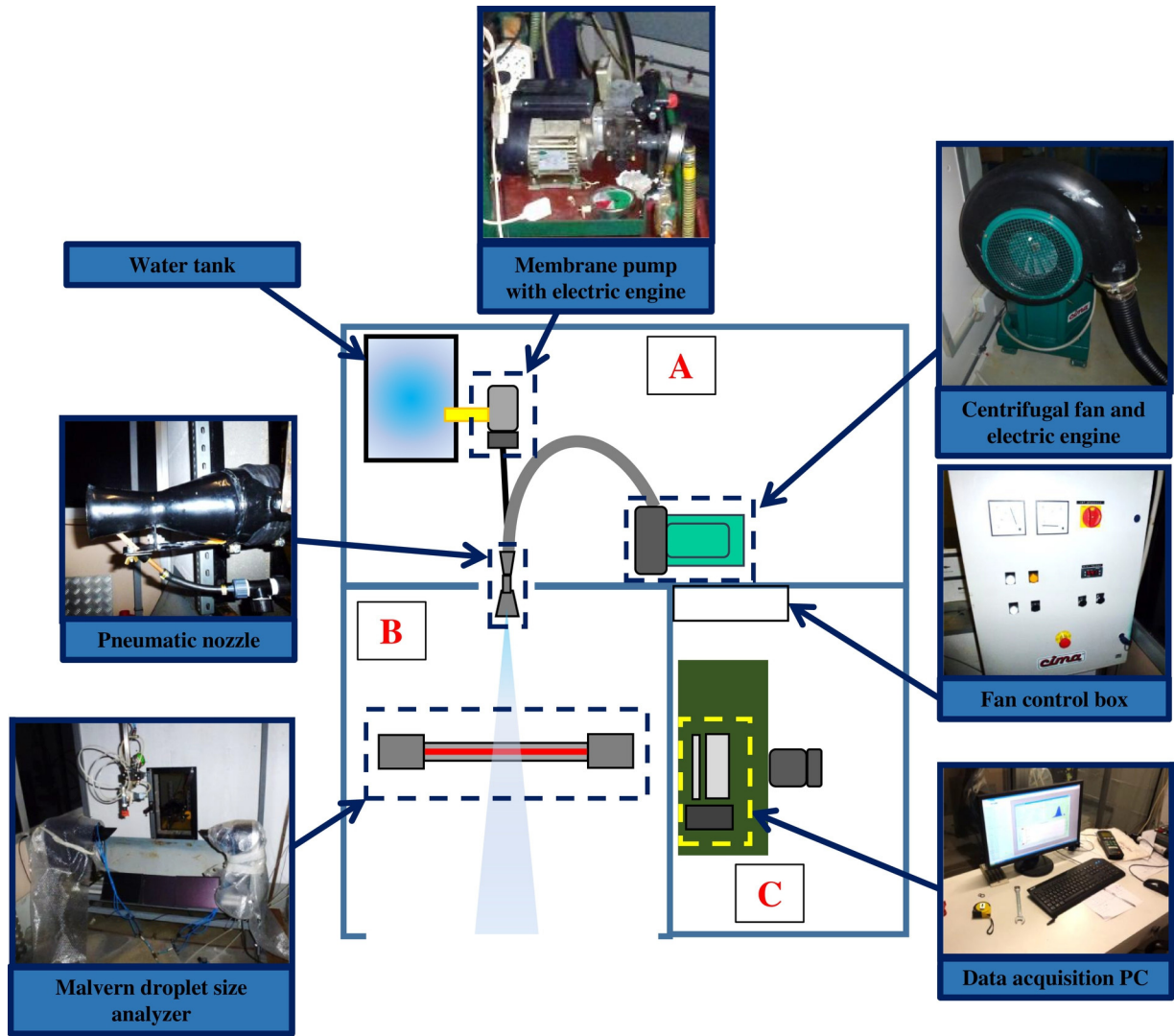
Fig. 1. Laboratory setup for the test bench and difference spaces: A. Spraying equipment, B. Spray droplet measurement instruments, and C. Trial control and data acquisition elements.
