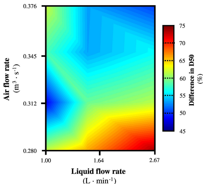
Fig. 11. Mean relative differences in D50 between the two liquid hose positions for every combination of AFR and LFR.
