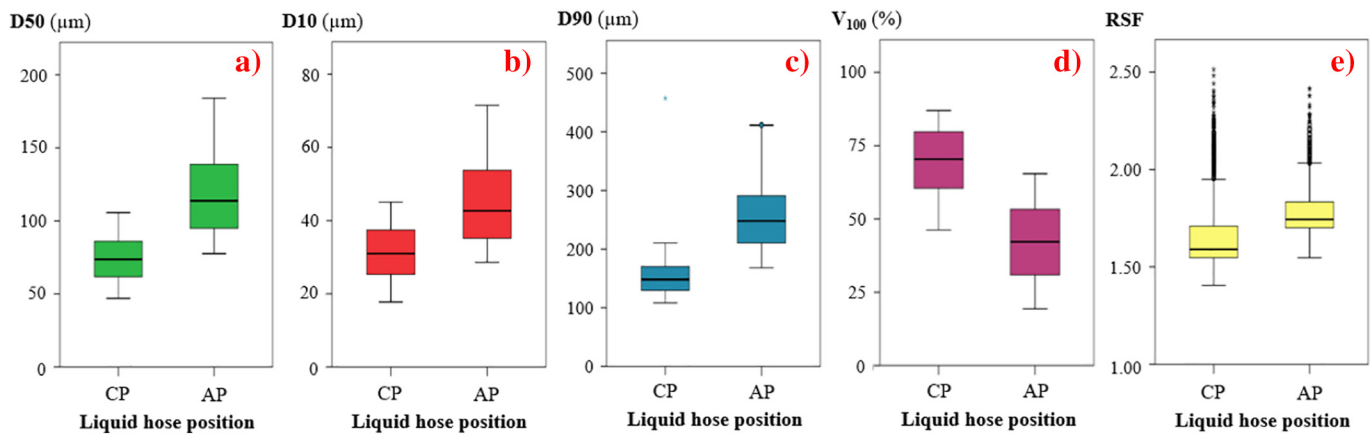
Fig. 9. Boxplots for the variables D50 (a), D10 (b), D90 (c), V_{100} (d), and RSF (e). The boxplots include all of the combinations of AFR and LFR considered.
