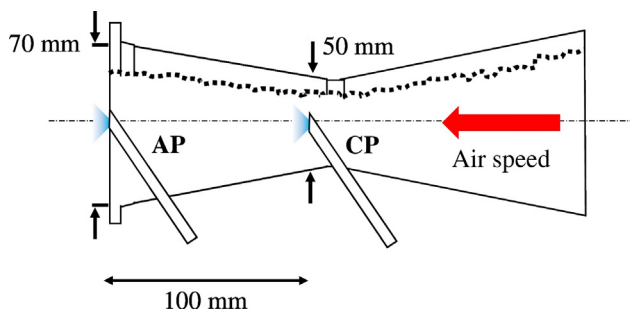
Fig. 3. Conventional (CP) and alternative (AP) positions of insertion of the liquid hose in the air spout.
