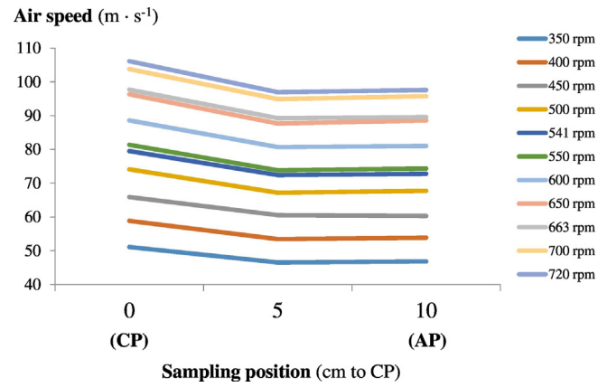
Fig. 8. Air speed values along the longitudinal axis of the air spout.
