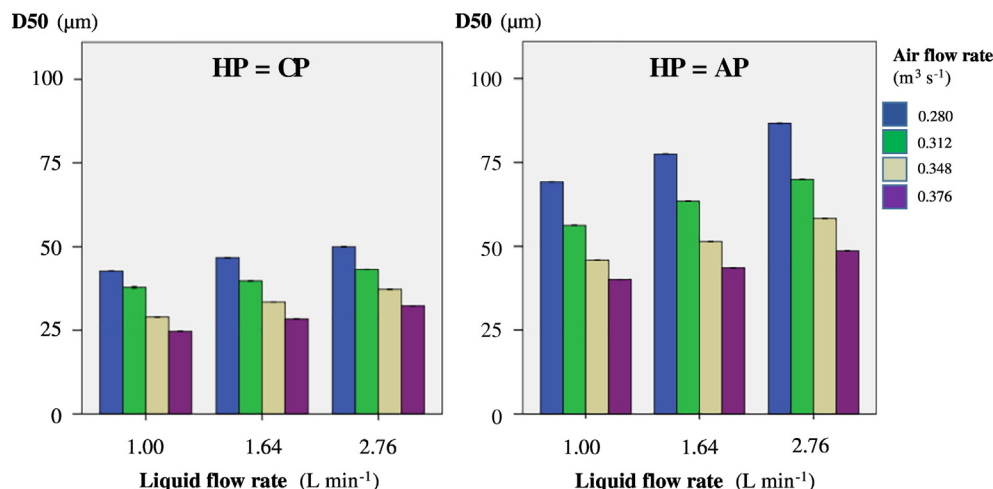
Fig. 10. D50 values for different combinations of variables for the two positions of the liquid hose. The error bars indicate the standard errors.
