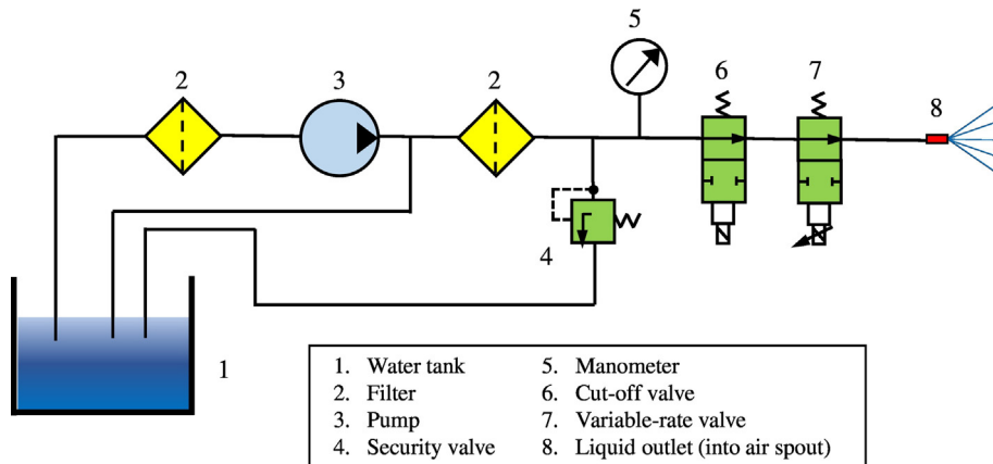
Fig. 2. Spraying circuit used in the test bench.
