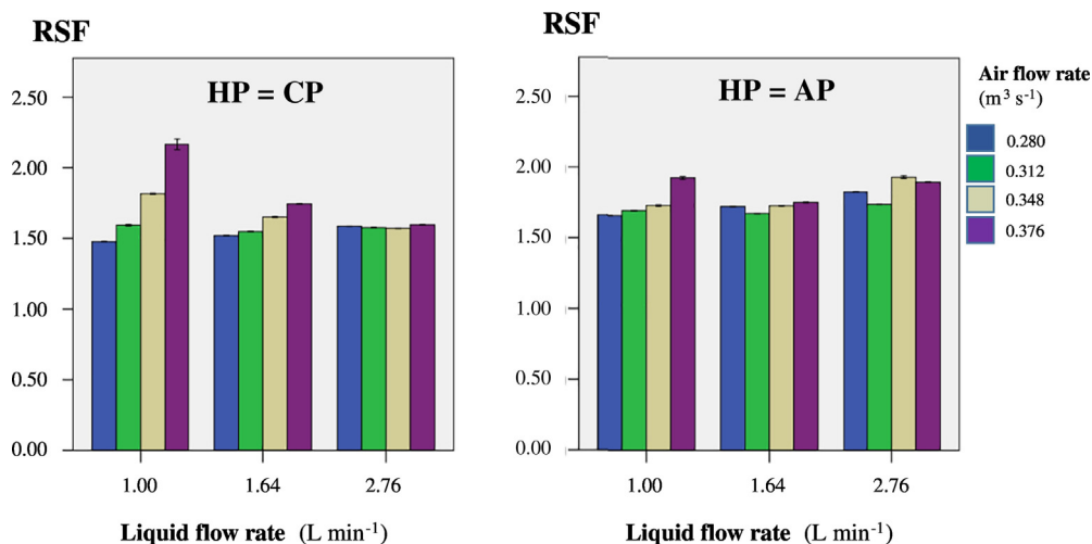
Fig. 13. Mean relative SPAN factor (RSF) for every tested combination of LFR and AFR for the two tested positions of the liquid hose. The error bars indicate the standard errors.
