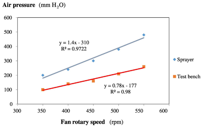
Fig. 7. Air pressure versus rotary speed for the sprayer and the test bench.
