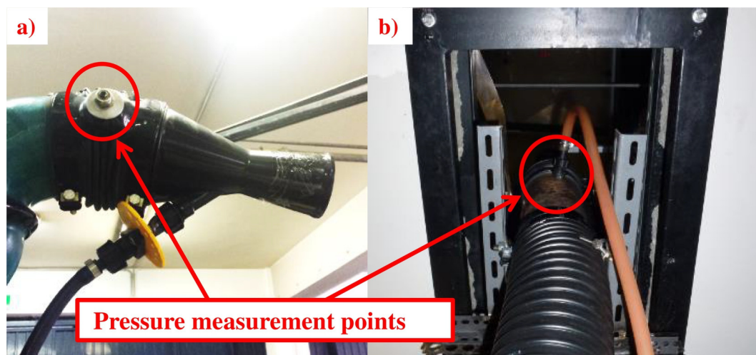
Fig. 4. Air pressure sampling position in: a) the real sprayer, and b) the prototype.
