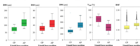
Droplet spectra measurements using laser spray diffraction system.
