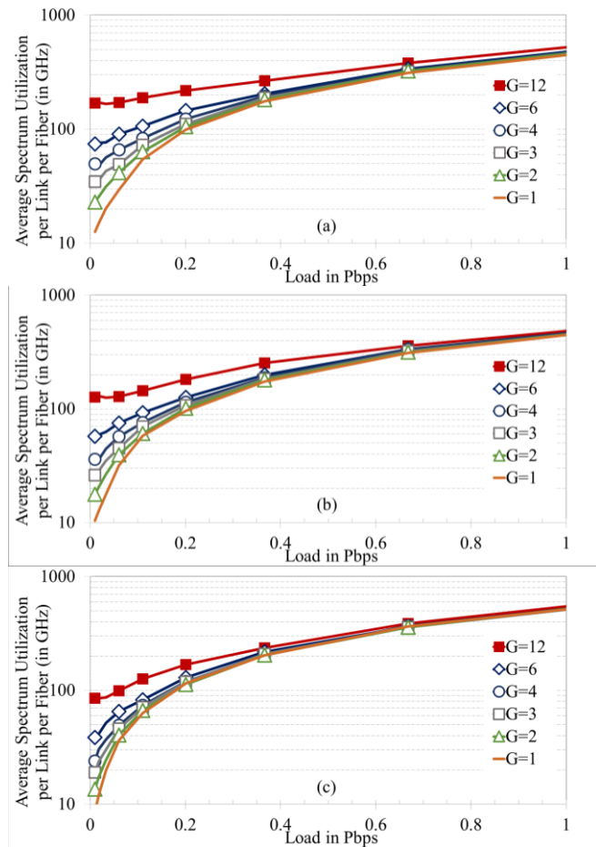
Fig. 6. Average spectrum utilization per link per fiber under different spatial Sp-Ch switching paradigms considering improved resolution WSS technology for (a) 50 GHz, (b) 37.5 GHz, and (c) 25 GHz ChBWs at a baud rate of 41, 28.5 and 16 Gbaud, respectively in terms of load.
