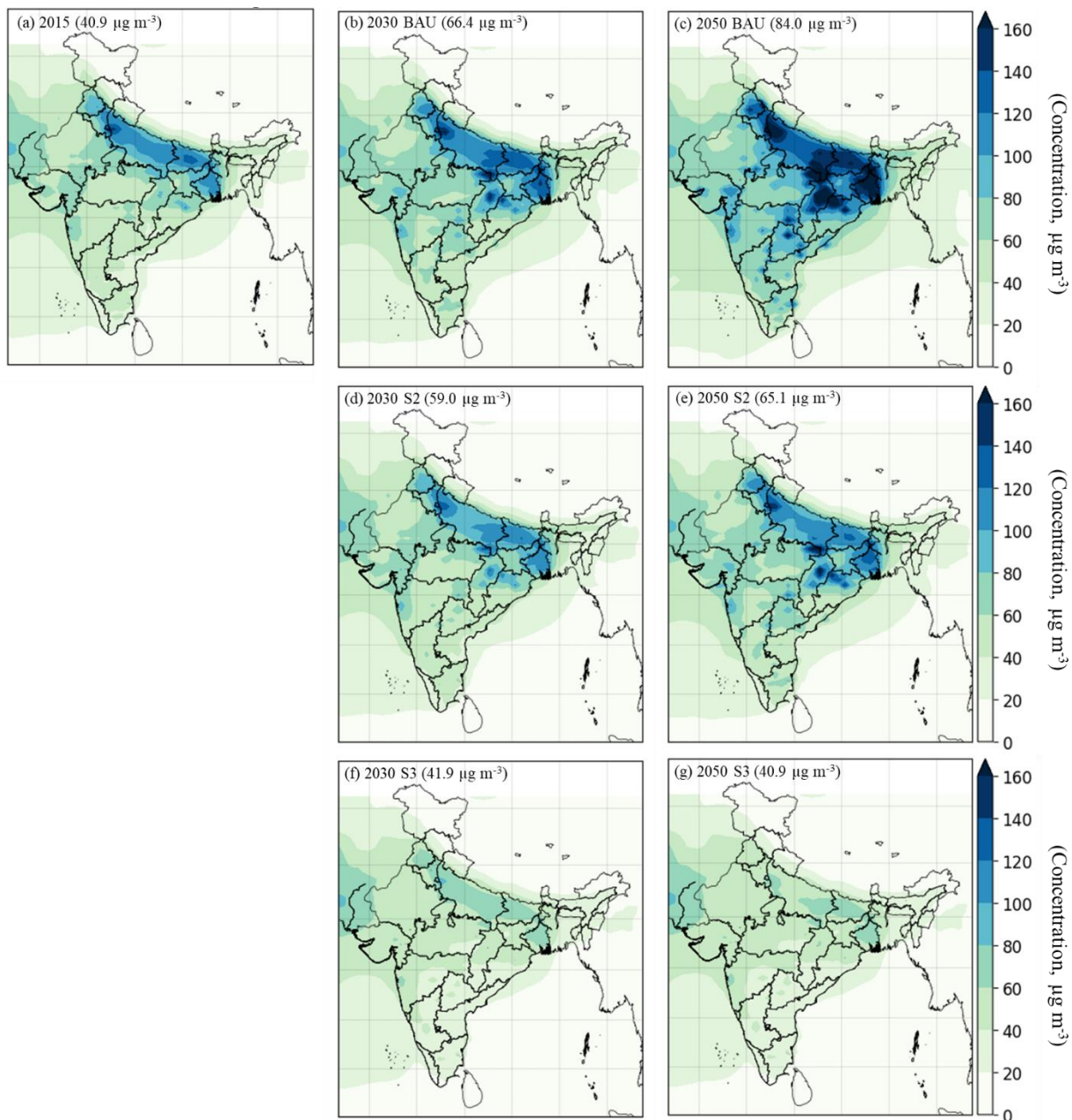
Figure 6. Simulated PM 2.5 concentration a) 2015 b) 2030 BAU c) 2050 BAU d) 2030 S2 e) 2050 S2 f) 2030 S3 g) 2050 S3. (Values in the parenthesis represent area-weighted average PM 2.5 concentration for India)
