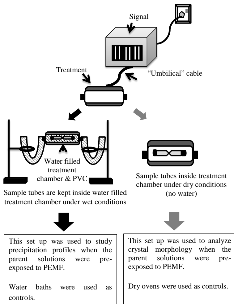
Figure 1 Schematics of the two different static PEMF testing set ups developed for the study of the commercial devices in either wet or dry testing conditions.
