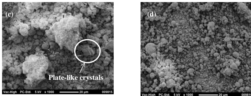
Figure 4: dried Dried precipitates from 1M parent solutions pre-exposed to (a) D PEMF (b) D control even (c) G PEMF (d) G control even for 30 min and mixed under at room temperature (22 °C).
