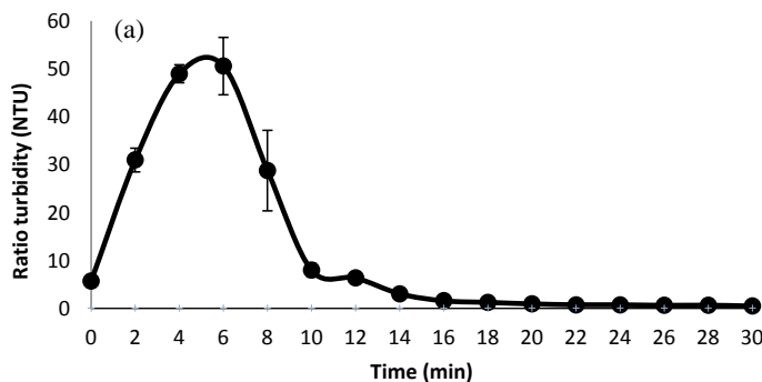
Figure 2 Establishment (b) precipitation profiles from the mixing of aqueous aqueous 5 mM \text{Na}_2\text{CO}_3 and \text{Ca}(\text{NO}_3)_2 \cdot 4\text{H}_2\text{O} over 30 min as a function (a) ratio turbidity (without PEMF involvement); error bars are standard errors for five replicates (b) UV absorbance at over 30 minutes as a function of absorbance at 350 nm (without PEMF involvement); error bars are standard errors in the mean for five replicates replicate experiments.
