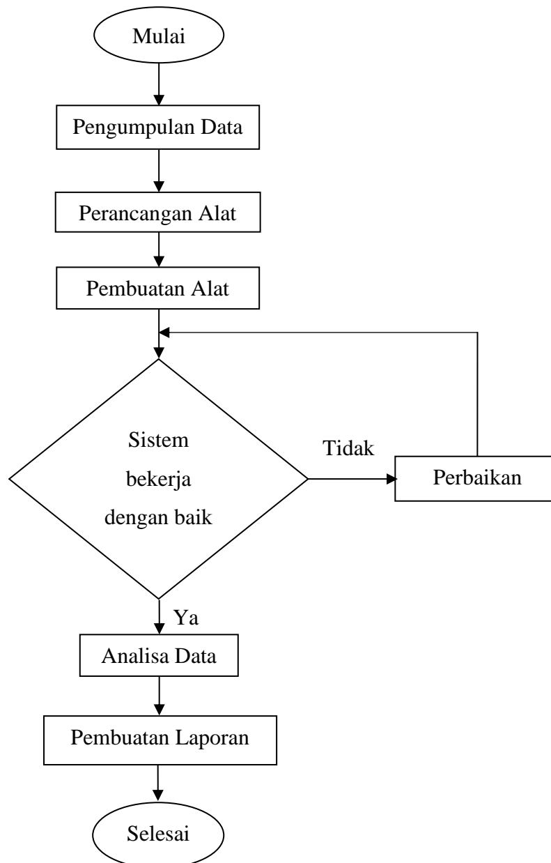
Gambar 1. Flowchart penelitian
