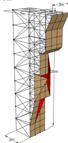
Gambar 3.5 Dinding Lead 3m x 18m
