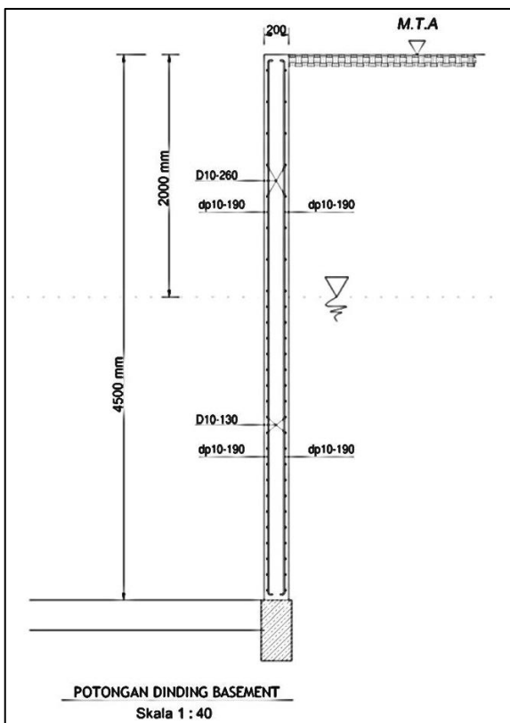
Gambar 4. Dinding basement
