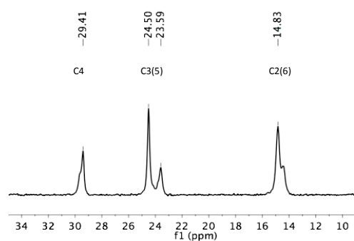
Figure 4. ^{13}\text{C} NMR spectrum of 1-cycano-1-sila-cyclohexane 4 at 110 K.
