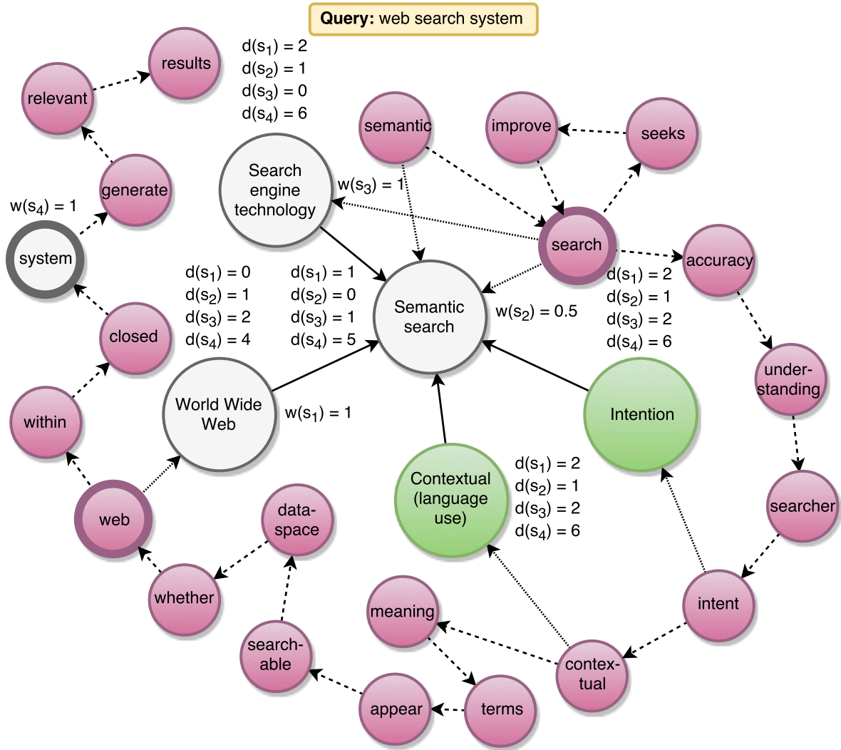
Figure 3.3: Searching for web search system over the graph-of-entity. Thicker node borders indicate query nodes, while light gray nodes correspond to identified seed nodes. We also show the confidence weight w(s) for each seed node, as well as the distances d(s) from seed nodes to each entity node.
