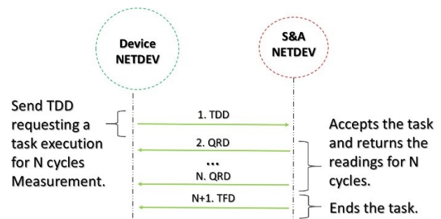
Figure 2. DIL Communication
