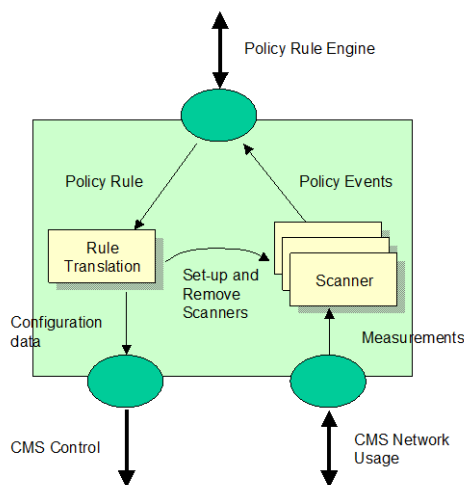
Figure 4 – CMS Provider.
