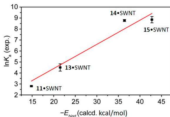
Figure 26. Plot of \ln K_a vs. -E_{bind} , comparing the experimental and calculated data.
