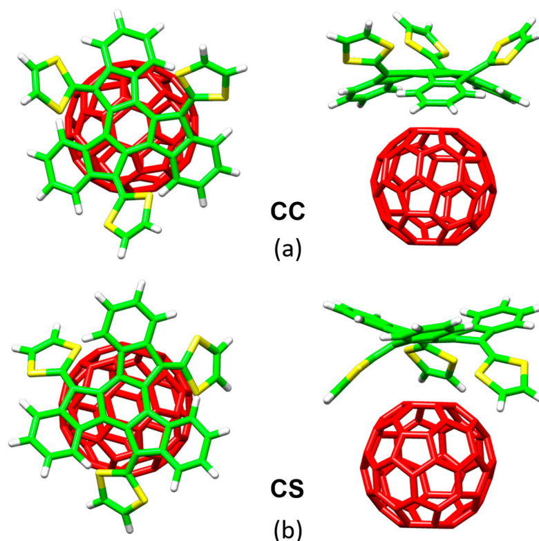
Figure 8. Minimum-energy structures of the truxTTF•C 60 complex calculated at the MPWB1K/6-31G** level. Top and side view of structures CC (a) and CS (b) are given. The
