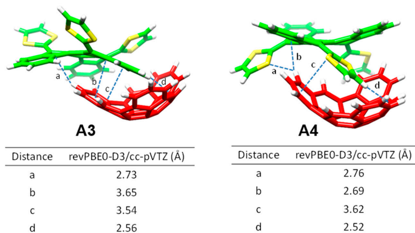
Figure 17. Selected intermolecular distances computed for structures A1–A4 at the revPBE0-D3/cc-pVTZ level. For C_{30}H_{12} , the carbon and hydrogen atoms are depicted in red and white, respectively. For truxTTF, the sulfur, carbon and hydrogen atoms are colored in yellow, green and white, respectively. Adapted with permission from [18]. Copyright 2014 WILEY-VCH Verlag GmbH & Co. KGaA.
