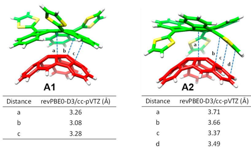
Figure 16. Minimum-energy structures ( A1 – 4 ) computed for the truxTTF• C_{30}H_{12} heterodimer at the revPBE0-D3/cc-pVTZ level. For C_{30}H_{12} , the carbon and hydrogen atoms are depicted in red and white, respectively. For truxTTF, the sulfur, carbon and hydrogen atoms are colored in yellow, green and white, respectively.
