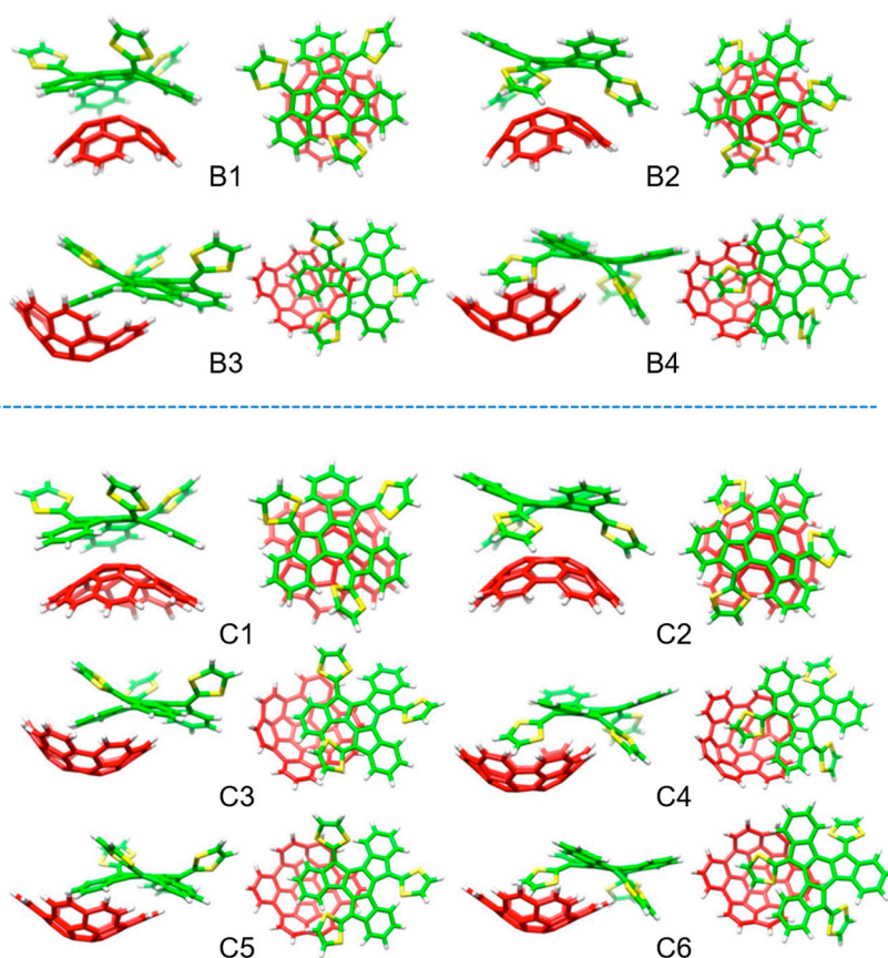
Figure 21. Minimum-energy structures and computed at the \text{revPBE0-D3/cc-pVTZ} level for the most stable conformations of the heterodimers formed by the \text{C}_{32}\text{H}_{12} (B1–4) and \text{C}_{38}\text{H}_{14} (C1–6) fullerene fragments with \text{truxTTF} ( \text{truxTT} \cdot \text{C}_{32}\text{H}_{12} and \text{truxTT} \cdot \text{C}_{38}\text{H}_{14} ). Except for the carbon atoms of the
