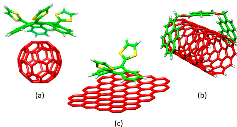
Figure 1. Selected examples of supramolecular assemblies involving fullerene (a), nanotubes (b) and graphene (c) with different \pi -conjugated electron-donors. The carbon atoms of the electron-acceptor carbon-based systems have been highlighted in red whereas the carbon atoms of the electron-donor systems are colored in green. Sulfur, oxygen and hydrogen atoms in the electron-donor systems are colored in yellow, red and white, respectively.
