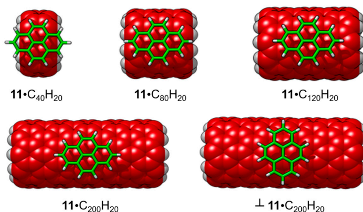
Figure 23. Minimum-energy geometries of parallel 11 •SWNT assemblies and the perpendicular 11 • C_{200}H_{20} calculated at the PBE0-D3/6-31G** level from a semi-rigid optimization with fixed intramolecular parameters (see the original Reference [117] for further details). Carbon atoms of SWNTs are highlighted in red whereas the carbon atoms of pyrene are in green. Hydrogen atoms are depicted in white. Reproduced from Reference [117] with permission from the Royal Society of Chemistry.
