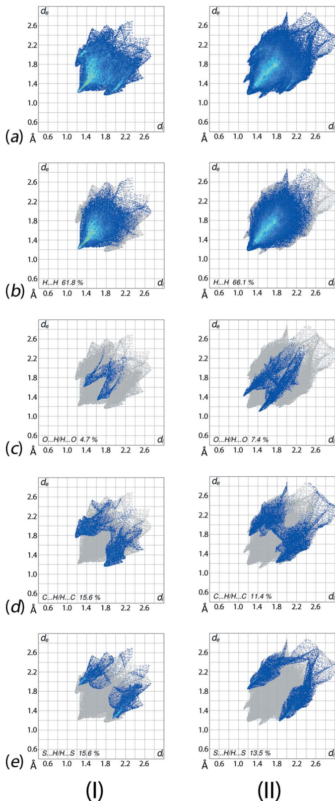
Figure 7 Comparison of the (a) complete Hirshfeld surface and full two-dimensional fingerprint plots between (I) and (II), and the plots delineated into (b) H...H, (c) O...H/H...O, (d) C...H/H...C and (e) S...H/H...S contacts.
