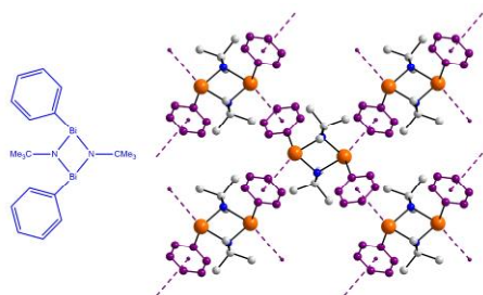
Figure X.15 Chemical diagram of [(t\text{-BuN})\text{BiPh}]_2 , ( 24 ), and the supramolecular layer sustained by \text{Bi}(\text{lp}) \cdots \pi(\text{arene}) interactions.
