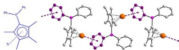
Figure X.5 Chemical diagram of \{(\eta^5\text{-diphenylphosphanyl-tetramethylcyclopentadienyl})\text{thallium}(\text{I}) , ( 5 ), and the supramolecular chain sustained by \text{Tl}(\text{lp})\cdots\pi(\text{arene}) interactions.
