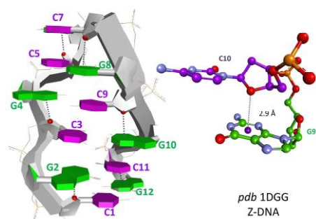
Figure X.23 Images highlighting the O(lp)···π(ring) interaction between the cytosine-sugarO(lp) and the pyrimidine ring of a guanine residue in left-handed Z-DNA.
