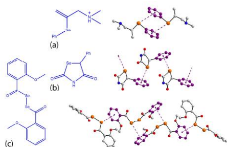
Figure X.16 Chemical diagrams of (a) [\text{MeSeC}(=\text{CH}_2)\text{CH}_2\text{N}^+(\text{H})\text{Me}_2] , ( 25 ), (b) 5-phenylselenazolidine-2,4-dione, ( 26 ), and (c) [2\text{-MeOC}_6\text{H}_4\text{C}(=\text{O})\text{Se}]_2 , ( 27 ), and their supramolecular aggregates sustained by \text{Se}(\text{lp}) \cdots \pi(\text{arene}) interactions.
