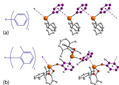
Figure X.14 Chemical diagrams of (a) \text{Ph}_3\text{Bi} , ( 22 ), and (b) \text{Bi}(\text{OC}_6\text{H}_3\text{Me}_2\text{-2,6})_3 , ( 23 ), and their supramolecular chains sustained by \text{Bi}(\text{lp}) \cdots \pi(\text{arene}) interactions.
