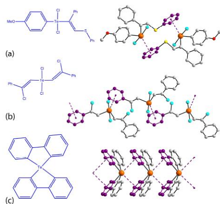
Figure X.22 Chemical diagrams of (a) (4\text{-MeOC}_6\text{H}_4)\text{Te}[(\text{Ph})\text{C}=\text{C}(\text{H})\text{SPh}]\text{Cl}_2 , ( 36 ), (b) [\text{Ph}(\text{Cl})\text{C}=\text{CH}]_2\text{TeCl}_2 , ( 37 ), and (c) bis(2,2'-biphenylene)-tellurium(IV), ( 38 ), and their supramolecular aggregates sustained by \text{Te}(\text{lp})\cdots\pi(\text{arene}) interactions.
