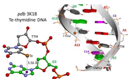
Figure X.24 Images highlighting the Te(lp)···π(ring) interaction of a doubly-bonded telluride atom interacting with the five-membered ring of a guanidine ring.
