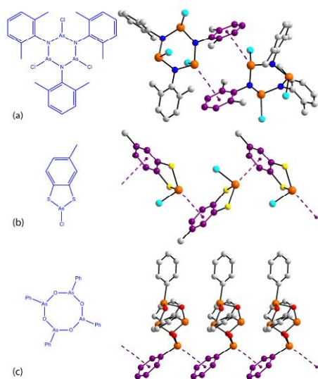
Figure X.10 Chemical diagrams of (a) [(2,6-Me 2 C 6 H 3 N)AsCl] 3 , ( 13 ), (b) chloro-(toluene-3,4-dithiolato)arsenic(III), ( 14 ), and (c) (PhAsO) 4 , ( 15 ), and supramolecular aggregates sustained by As(lp)···π(arene) interactions.
