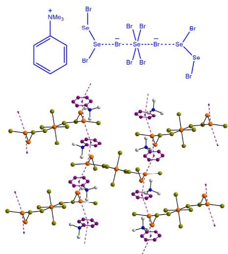
Figure X.19 Chemical diagram of [\text{PhN}^+\text{Me}_3][\text{SeBr}_4]\{2[\text{Se}_2\text{Br}_2].2\text{Br}^-\} , ( 33 ), and the supramolecular layer sustained by \text{Se}(\text{lp}) \cdots \pi(\text{arene}) interactions.
