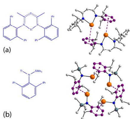
Figure X.4 Chemical diagrams of (a) [2-(2',6'\text{-di-isopropylphenylamido})-4-(2',6'\text{-diisopropylphenylimino})-2\text{-pentene}]\text{thallium}(\text{I}) , ( 3 ), and (b) \text{Tl}[\text{N}(\text{SiMe}_3)\text{C}_6\text{H}_3(\text{iPr})_2-2,6] , ( 4 ), and supramolecular aggregates sustained by \text{Tl}(\text{lp})\cdots\pi(\text{arene}) interactions. Additional colour code: hunter green, silicon; blue, nitrogen.
