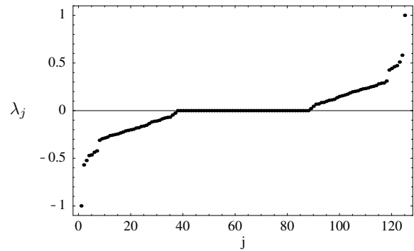
Figure 2: Eigenspectrum of the ontology sorted by value
