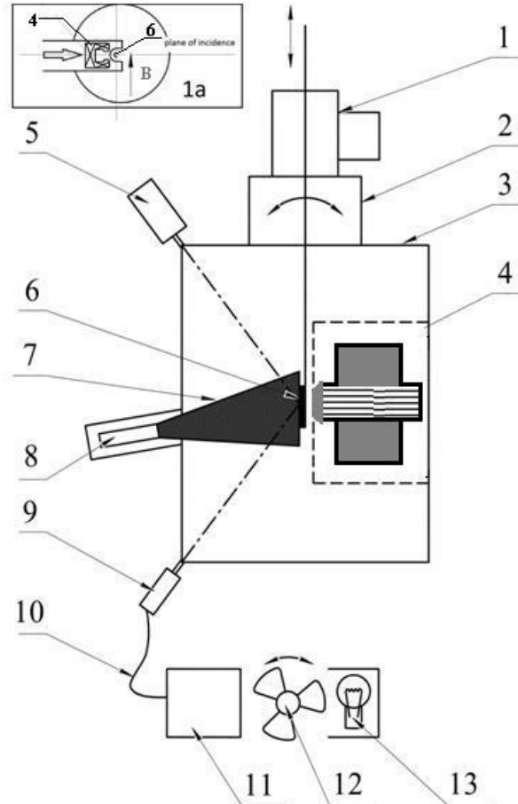
Figure 1: Schematic diagram of the experimental setup (1 – substrate introduction chamber, 2 – substrate rotation control, 3 – main UHV chamber, 4 – electromagnet 400 mT, 5 – analyzer part, 6 – sample, 7 – molecular beam, 8 – evaporator, 9 – polarizer part, 10 – optic cable, 11 – spectroscope, 12 – shutter for creation the sync-pulse, 13 – light source)
