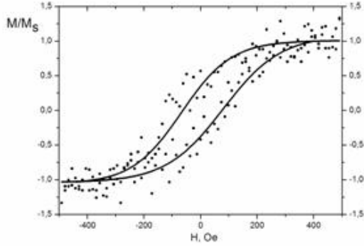
Figure 4: The hysteresis loop obtained for Fe/SiO_2/Si by means of magneto-ellipsometry.
