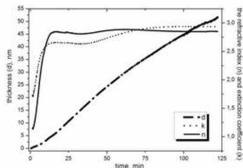
Figure 2: The thickness (d), the refractive index (n) and extinction coefficient (k) of Fe film obtained as function of the evaporation time and calculated during the process of Fe/SiO_2/Si thin film synthesis
