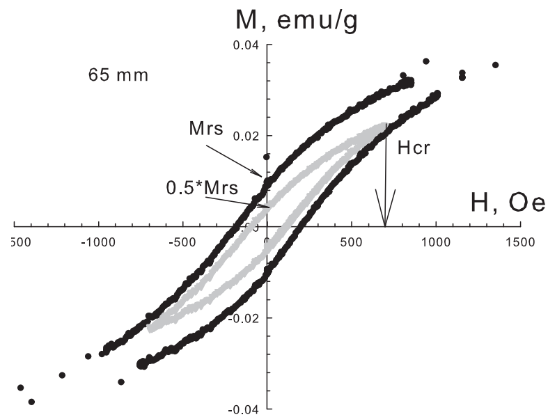
Fig. 1. Typical results of magnetic measurements of a sediment at the depth of 65 mm together with FM and PM contributions
